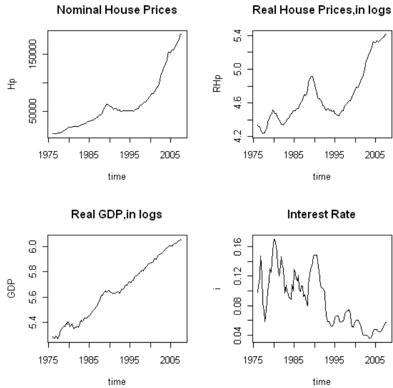
Figure 3: Series
