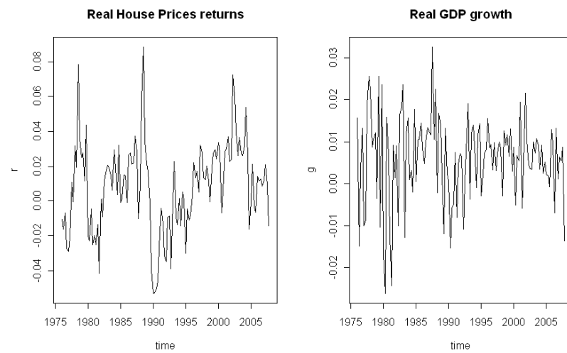
Figure 4: Series
