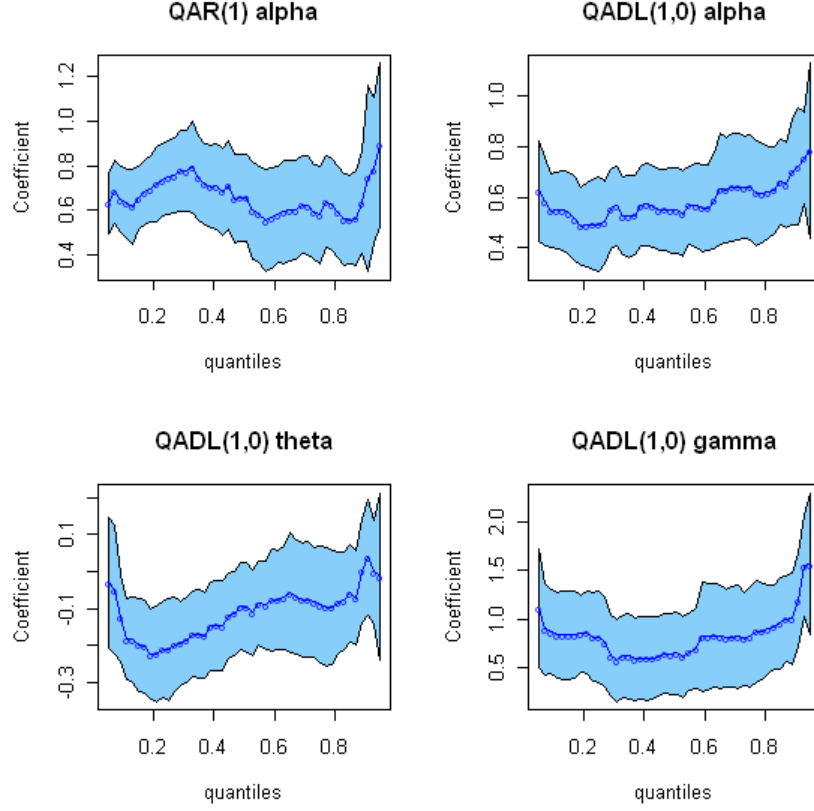
Figure 5: Coefficient estimates
