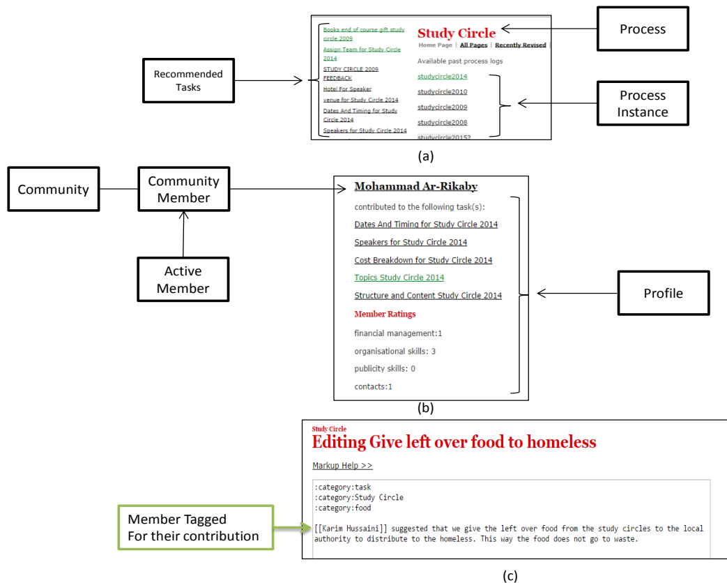
Fig.4.3 Pimki tool mapped to Social BPM design
