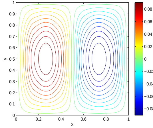
(f) N_{cr} = 32.012 , S-C-S-C
