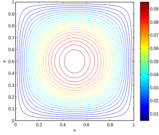
(a) N_{cr} = 26.320 , S-S-S-S
