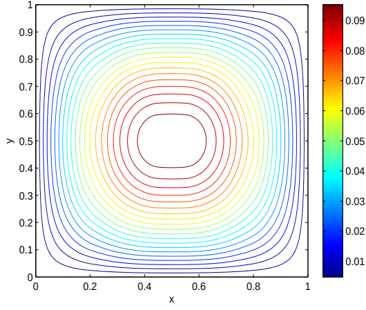
(a) N_{cr} = 27.767 , S-S-S-S
