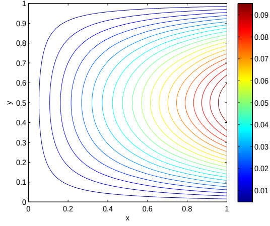
(b) N_{cr} = 8.9501 , S-S-S-F
