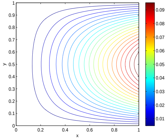
(e) N_{cr} = 10.769 , S-C-S-F
