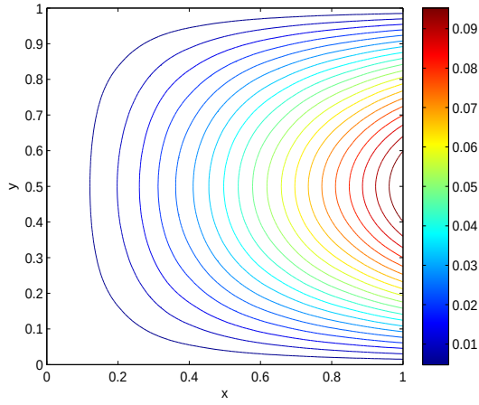
(e) N_{cr} = 11.373 , S-C-S-F
