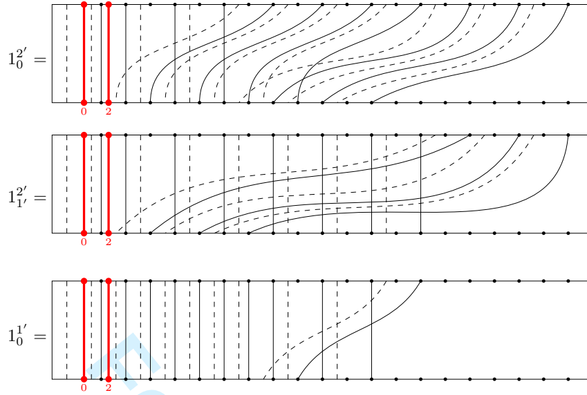
Fig. 25: The elements 1_0^{2'} , 1_0^{1'} , and 1_1^{2'} corresponding to the paths in Figure 24.
