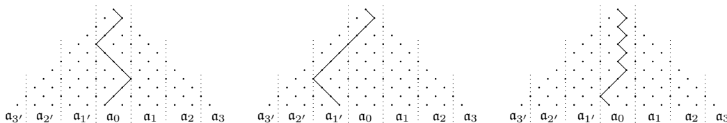
Fig. 24: Some examples of maximal paths (of degree 2, 1, and 1 respectively).
