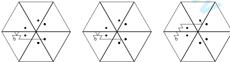
Fig. 4: The unique paths in \text{Path}((2, 9, 2), \omega^\gamma) , in \text{Path}((2, 8, 3), \omega^\gamma) , and in \text{Path}((5, 8, 0), \omega^\gamma) of degrees 1, 2, and 1 respectively.
