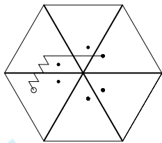
Fig. 2: Our fixed path \omega^\gamma from the origin to \gamma = (4, 9, 0) . (The space has been cropped to only include points less than or equal to \gamma in the dominance ordering.)
