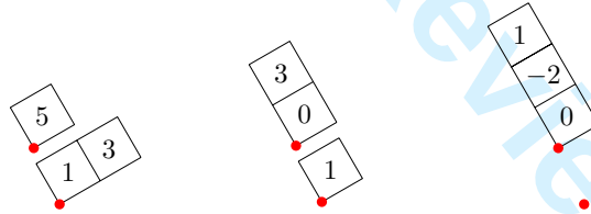
Fig. 15: The semistandard tableaux T \in \text{SStd}(((1), (1^2)), (\emptyset, (1^3))) , U \in \text{SStd}(((2), (1)), ((1), (1^2))) , and V \in \text{SStd}(((3), \emptyset), ((2), (1))) , respectively.
