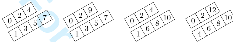
Fig. 21: These semistandard tableaux are of weights ((1^3), (1^4)) , ((1^2), (1^5)) , ((1^6), (1)) and ((1^7), \emptyset) respectively. The tableaux are of degrees 0, 1, 1, and 2 respectively.
