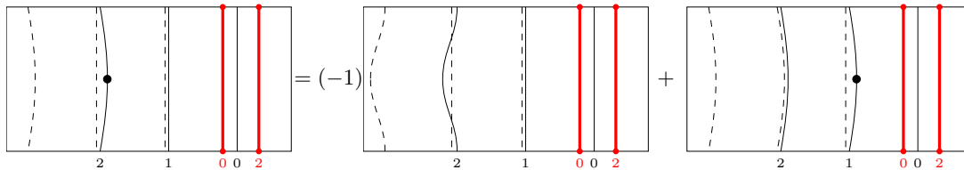
Fig. 19: The two terms obtained by applying relation (2.7) to the rightmost diagram in Figure 18.
