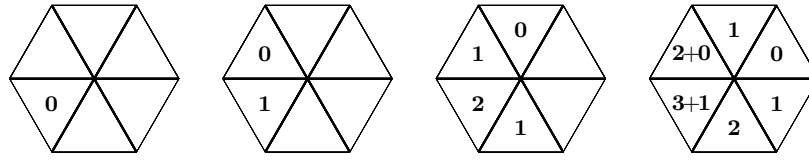
Fig. 10: The first four steps of running Soergel's cancellation-free algorithm along \omega^\gamma . We have recorded the powers of the polynomials only (for example, 2 + 0 should be read as t^2 + t^0 ).
