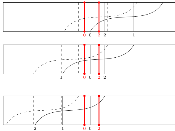
Fig. 16: The basis elements corresponding to the tableaux T , U , and V in SStd(((1), (1^2)), (\emptyset, (1^3))) , SStd(((2), (1)), ((1), (1^2))) , and SStd(((3), \emptyset), ((2), (1))) , respectively (see Figure 15).
