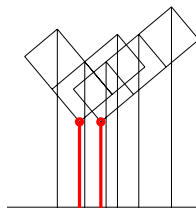
Fig. 12: The diagram and loading of the bipartition ((2, 1), (1^3)) for \ell = 2 , g = 1 , \theta = (0, 0.5) .
