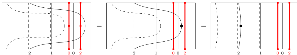
Fig. 18: The product (B_V)^*(B_V) . The first equality follows from relations (2.11); the second follows from relations (2.5) and (2.11).
