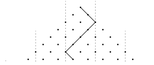
Fig. 22: The path \omega(T) \in \text{Path}((3, 4), \omega^{(7,0)}) .
