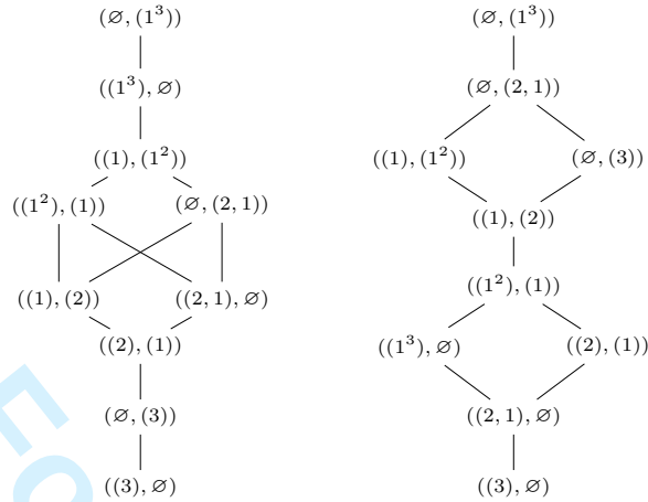
Fig. 14: The Hasse diagrams of the posets corresponding to the FLOTW and well-separated weightings.
