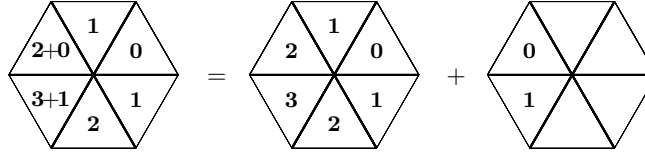
Fig. 11: Rewriting the m_{\omega^\gamma}(\lambda) in terms of n_\mu(\lambda) and e_{\omega^\gamma}(\mu) .
