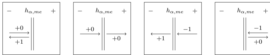
Fig. 6: The four subcases for the values of d_\alpha(\omega, k) as \omega crosses a wall. The \pm indicate the distinct subsets E_r^+ and E_r^- of E_r . In each case the first (respectively second) step has its degree recorded as a superscript (respectively subscript).
