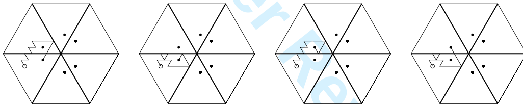
Fig. 3: The leftmost two paths are in \text{Path}(\alpha, \omega^\gamma) and are of degrees 1 and 3 respectively. The final two paths are the elements of \text{Path}(\beta, \omega^\gamma) and are of degrees 0 and 2, respectively.
