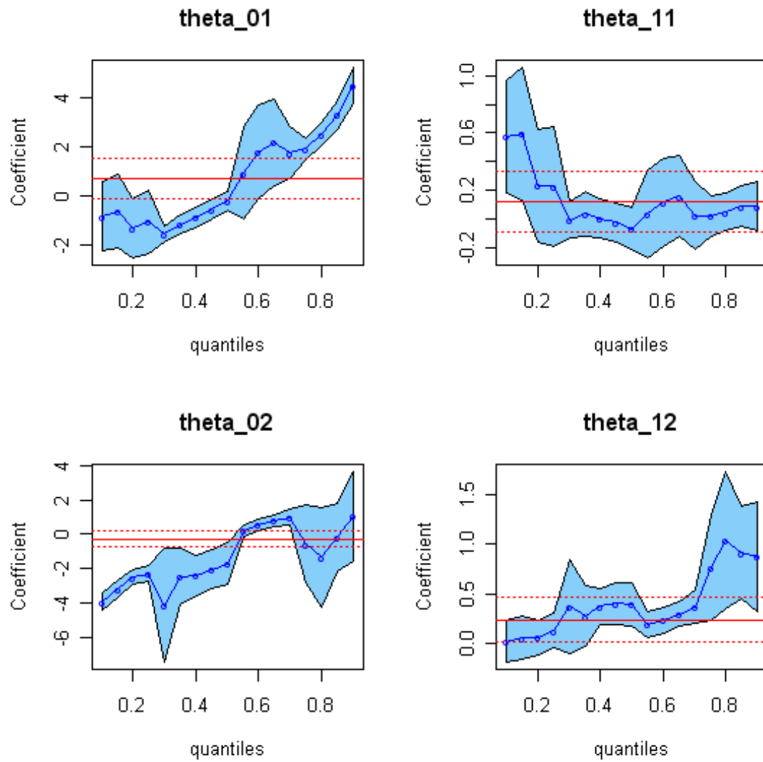
Figure 3: Parameter estimates: OLS and QR
