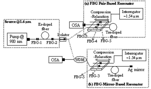
Fig. 2. Schematic diagram of tunable laser resonator (a) created by FBG pair and (b) created by an HR FBG and an LR broadband mirror at the fiber end. FBG-1, 99.9% HR FBG at 1.6 \mu\text{m} ; FBG-2, 26% LR FBG at 1.6 \mu\text{m} ; FBG-3, 99.9% HR FBG at 1.997 \mu\text{m} ; FBG-4, 80% LR FBG at 1.997 \mu\text{m} ; FBG-5, reference FBG at 1.548 \mu\text{m} .
