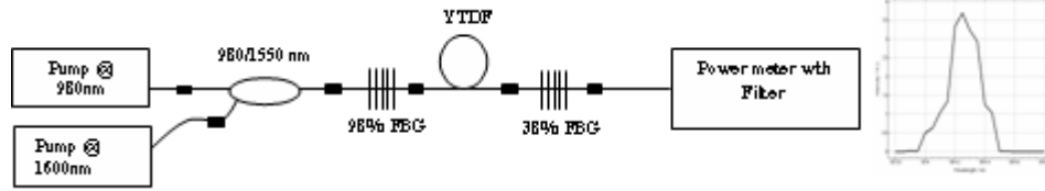
Fig. 2. Schematic of Laser set up at 1874 nm using \text{Yb}^{3+} sensitized \text{Tm}^{3+} doped fiber. Laser spectrum recorded in monochromator is shown in inset.
