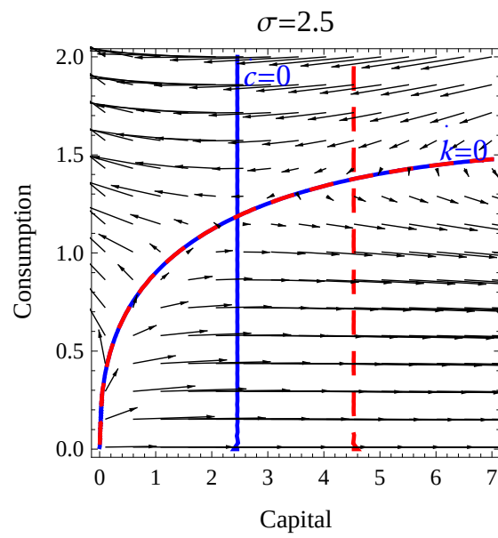
Figure 3: Vector field following the doubling of the tax on capital income.
