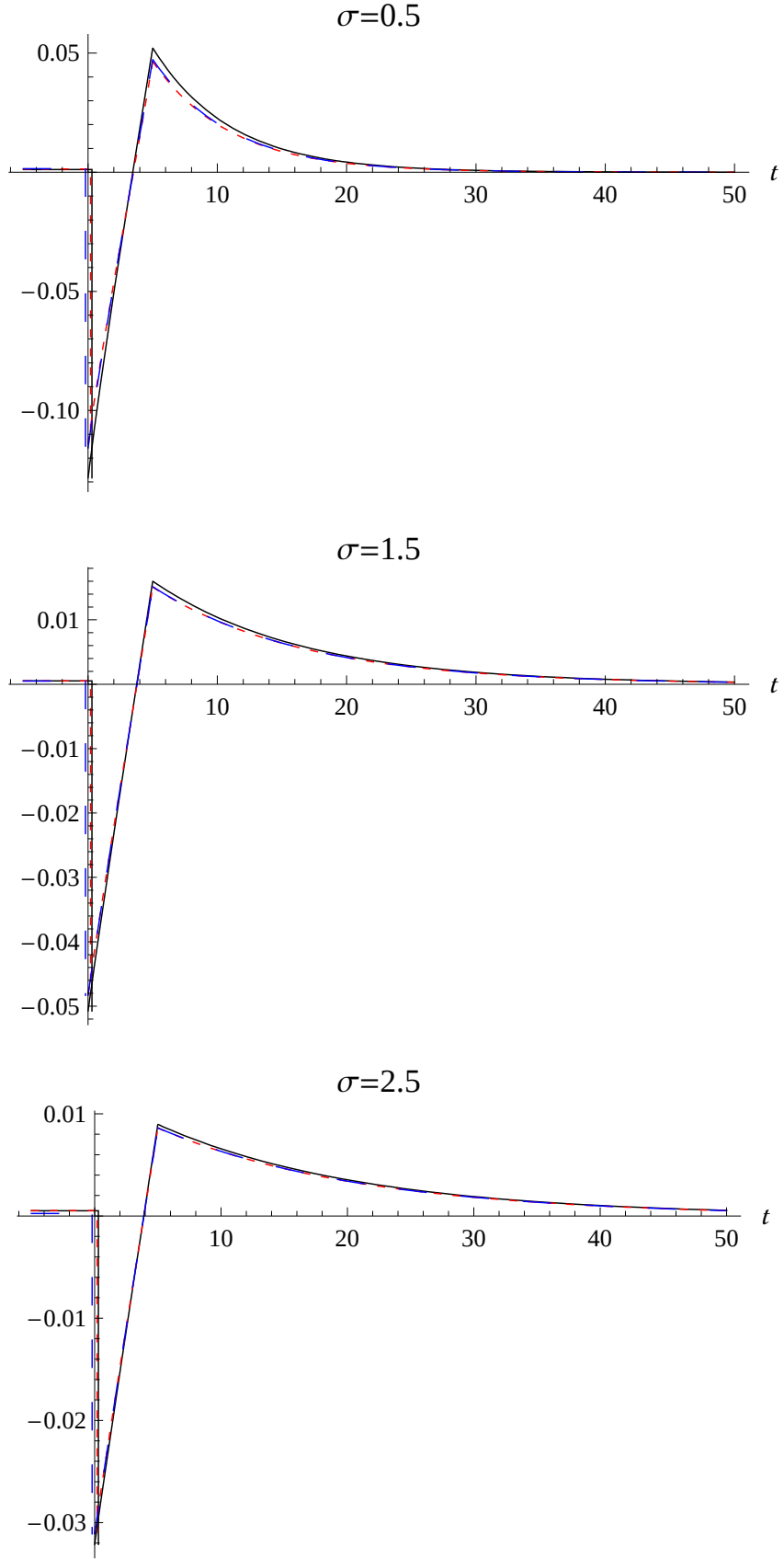
Figure 12: The behavior of consumption following the reduction of the tax on income from capital from 0.35 to zero for T = 5 years. The solid black curve represents a first order approximation, the curve with small red dashes, a second order approximation, the large blue dashes, a third order approximation.
