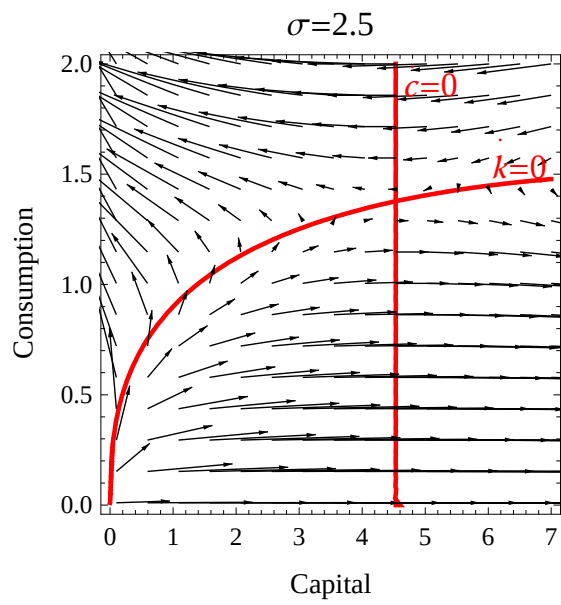
Figure 1: Vector field for the baseline model with \tau = 0.35 .
