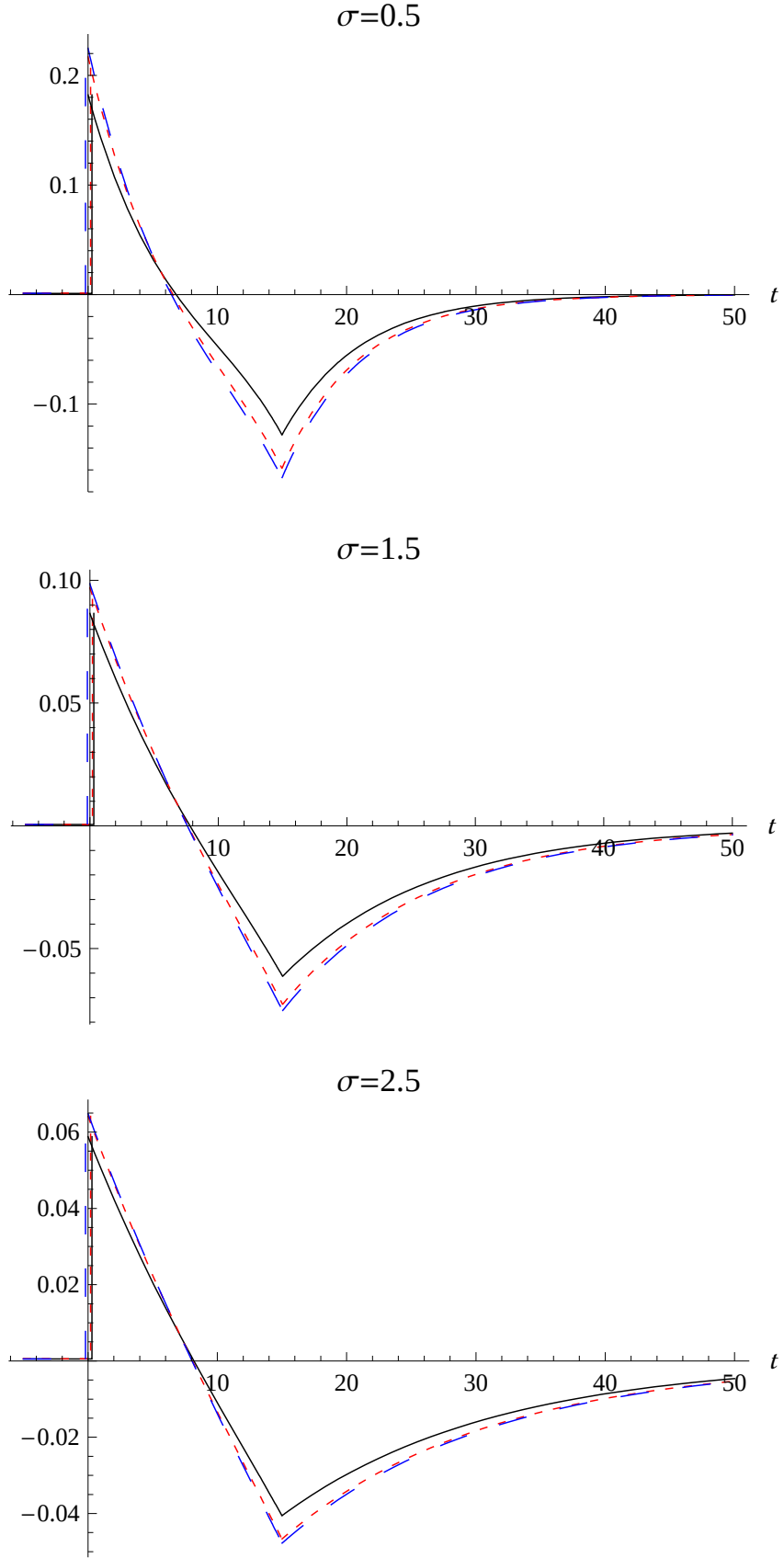
Figure 10: The behavior of consumption following the doubling of the tax on income from capital from 0.35 to 0.7 for T = 15 years. The solid black curve represents a first order approximation, the curve with small red dashes, a second order approximation, the large blue dashes, a third order approximation.
