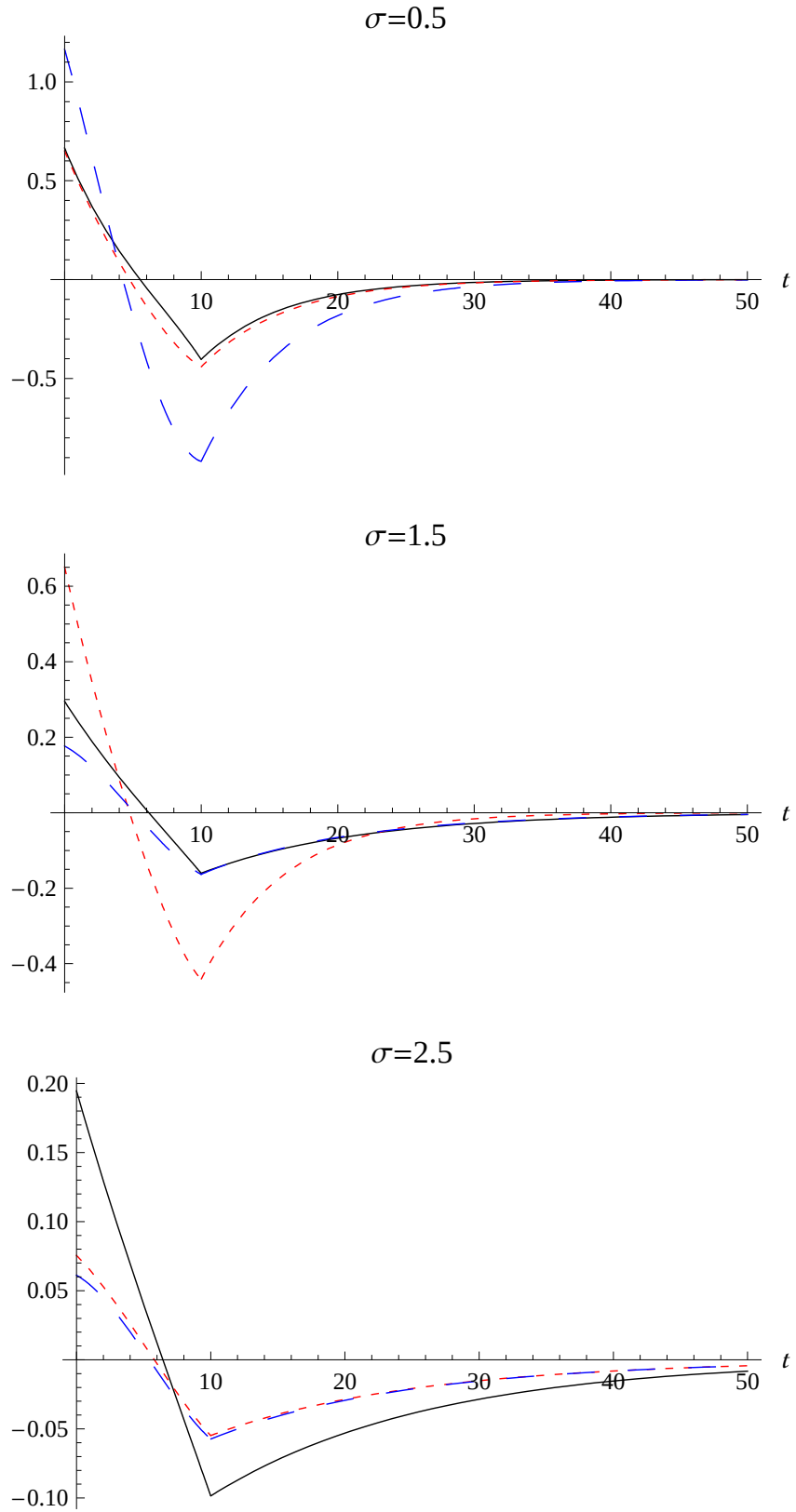
Figure 5: The first three moments of the approximation of consumption, c_\epsilon(t) (solid black curve), c_{\epsilon\epsilon}(t) (small red dashes), and c_{\epsilon\epsilon\epsilon}(t) (large blue dashes), for T = 10 and \sigma = 0.5, 1.5, 2.5 .
