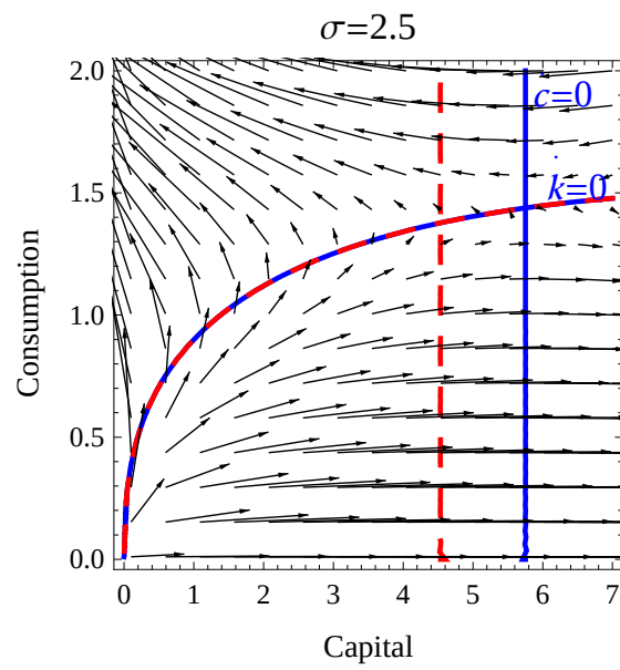
Figure 2: Vector field following abolition of the tax on capital income.
