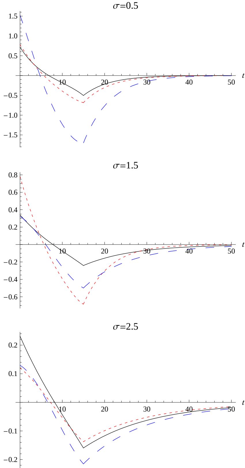
Figure 6: The first three moments of the approximation of consumption, c_\epsilon(t) (solid black curve), c_{\epsilon\epsilon}(t) (small red dashes), and c_{\epsilon\epsilon\epsilon}(t) (large blue dashes), for T = 15 and \sigma = 0.5, 1.5, 2.5 .
