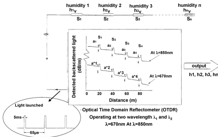
Fig. 6. Optical responses of distributed fibre-optic sensing system using optical time domain reflectometer (OTDR) [34].
