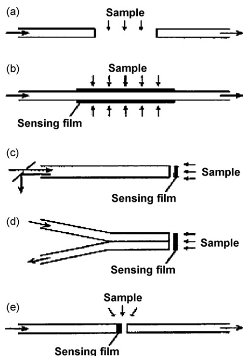
Fig. 2. Various configurations for spectroscopic fibre-optic sensors [16].
