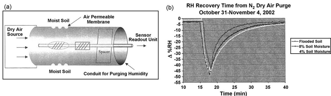
Fig. 11. (a) Schematic of a polymer-coated FBG sensor for soil moisture sensing. (b) Data showing evaporation rate of soil samples with various moisture content [60].
