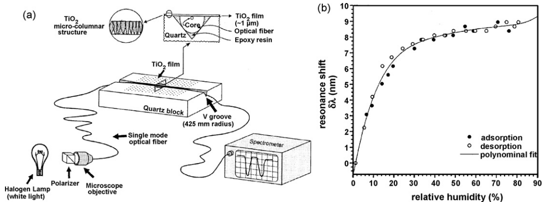
Fig. 10. (a) Experimental set-up for monitoring humidity-induced resonance band shift of a side-polished optical fibre with \text{TiO}_2 overlay. (b) Sensor response to humidity measured using resonance at 633 nm [48].
