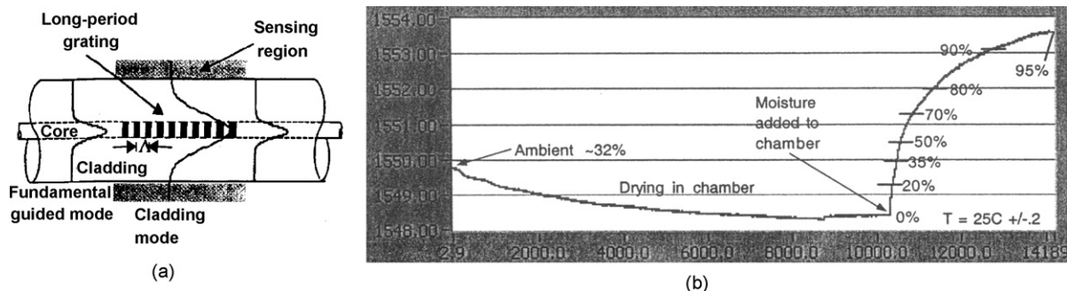
Fig. 13. (a) Schematic of a LPG sensor. (b) Sensing characteristics of a CMC-coated LPG humidity sensor [63].
