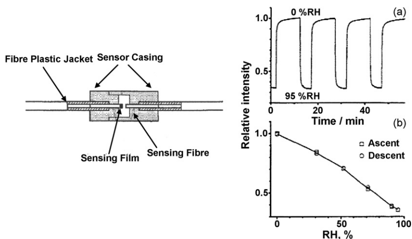
Fig. 4. Sensing characteristics of a fibre-optic humidity sensor using the air-gap configuration [16].
