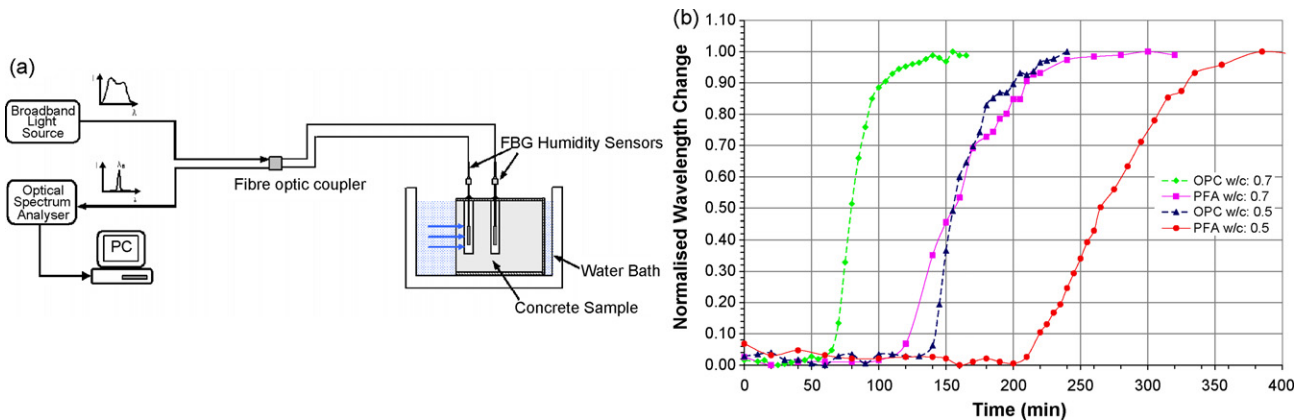
Fig. 12. (a) Experimental set-up used for moisture ingress rate measurement using FBG humidity sensors. (b) Sensor measurements showing moisture ingress characteristics of various concrete specimens using sensor positioned at 25 mm away from cube face [62].
