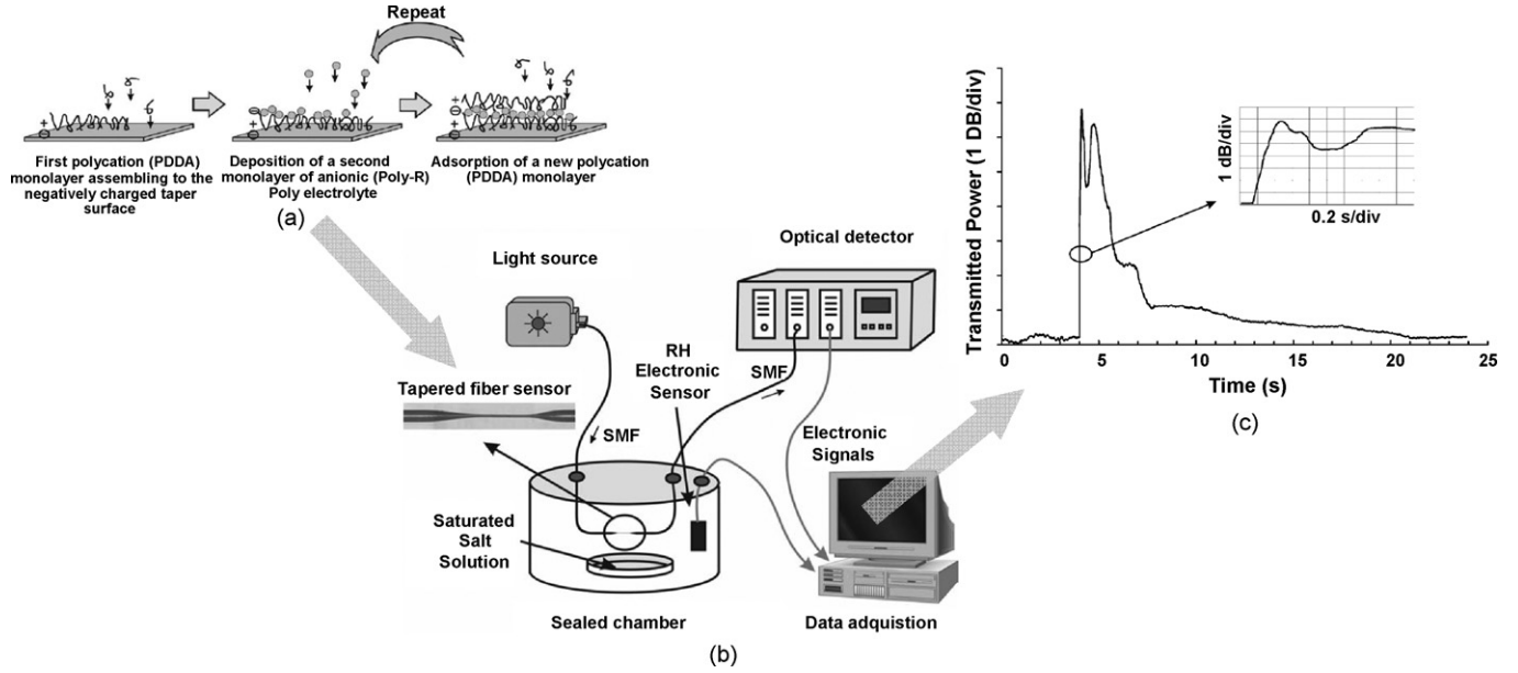
Fig. 9. Tapered optical fibre humidity sensor with ISAM overlay. (a) Schematic of ISAM deposition process. (b) Experimental set-up for sensor characterisation. (c) Sensor response to a short abrupt change of humidity simulated by human breath [45].
