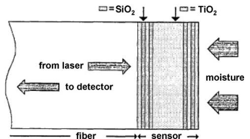
Fig. 15. FO Fabry–Perot interferometric humidity sensor [73].
