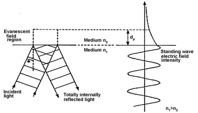
Fig. 5. Evanescent field generated at the interface of two optically transparent media [29].
