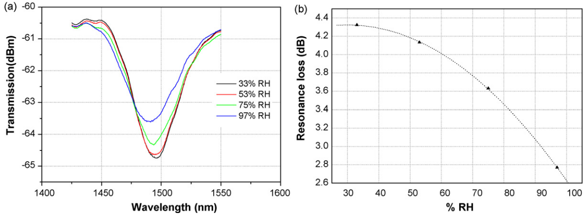
Fig. 14. (a) Spectral characteristics of PVA-coated LPG at 1500 nm. (b) Transmission dip variation at various RH levels [68].
