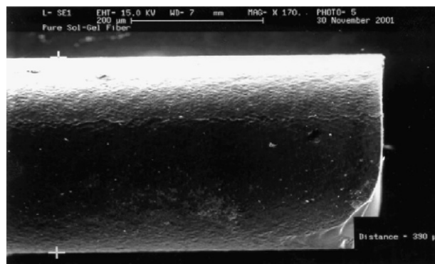
Fig. 3. SEM picture of the porous sol-gel silica fibre, showing the interconnected porous structure on the surface of the fibre [14].
