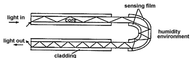
Fig. 7. U-bent evanescent wave sensor configuration using cladding as the active sensing region [35].
