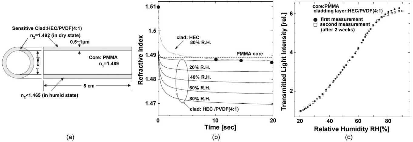
Fig. 8. Evanescent wave POF humidity sensor using PMMA core and HEC/PVDF film. (a) Sensor configuration. (b) Refractive index change of HEC/PVDF film at various humidity conditions. (c) Sensor characteristics [41].
