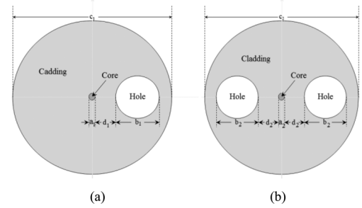
Fig. 1. (a) One-hole high-birefringence fiber that has a hole diameter b_1 of 30\text{ }\mu\text{m} and the distance between the right edge of the core to the left edge of the hole d_1 is 9\text{ }\mu\text{m} . (b) Two-hole high-birefringence fiber that has two holes with the same diameter b_2 of 27\text{ }\mu\text{m} and the distance between the right edge of the core to the left edge of the hole on the right d_2 is 14\text{ }\mu\text{m} .
