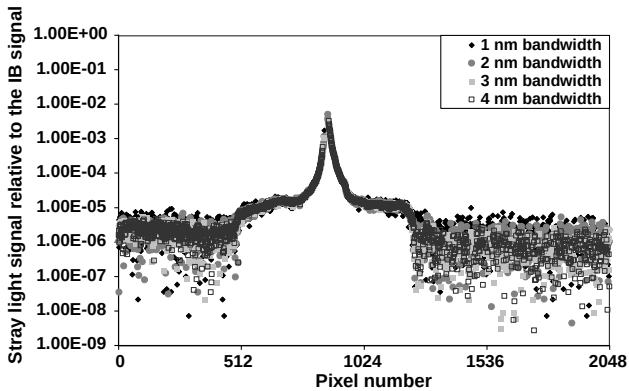
Fig. 5. Spectral stray light distribution function for different monochromator bandwidths.
