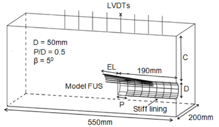
Figure 4. Model test apparatus.
