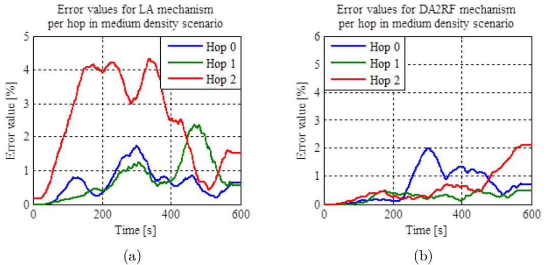
Figure 5.24: Per hop error values for the LA (a) and the DA2RF (b) mechanisms in medium density scenario.
