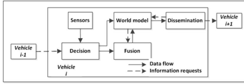
Figure 4.1: Generic data aggregation modelling for VANETs.
