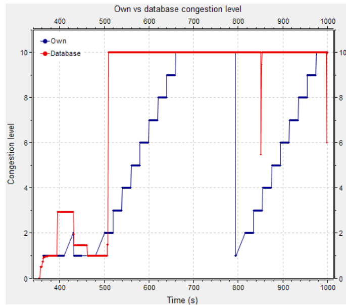
Figure 4.8: Detected values of congestion on the vehicle's route.
