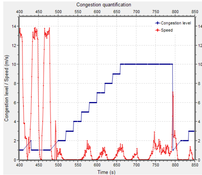
Figure 4.6: Congestion quantification process.
