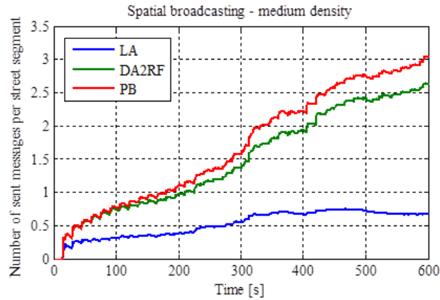
Figure 5.13: Spatial Communication in medium density scenario for the LA , DA2RF and PB mechanisms.
