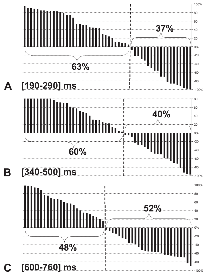
FIG. 5. Distribution of the LFP amplitude during the first (A), second (B) and third (C) activity periods normalized to the contact pair with the maximum amplitude from each electrode (in the standard motor task). Negative values indicate polarity inversion relative to the sign of the contact pair with the maximum amplitude (defined as +100%).
