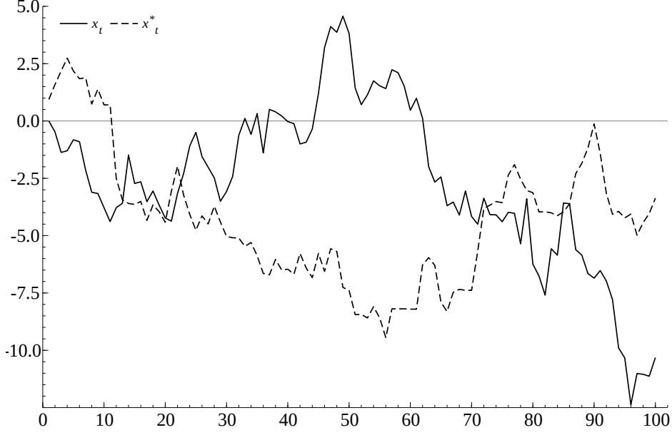
Figure 5: MEBB sample path replication.
