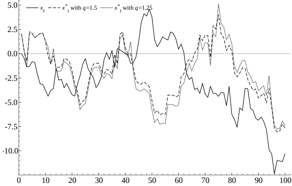
Figure 10: MnEBB sample path replication.
