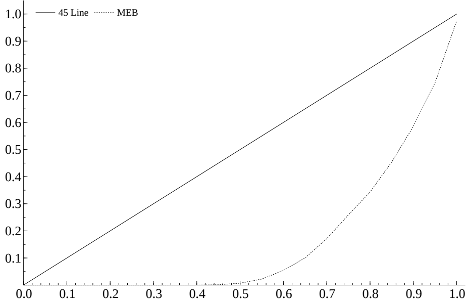
Figure 2: Empirical rejection frequencies of the MEB.
