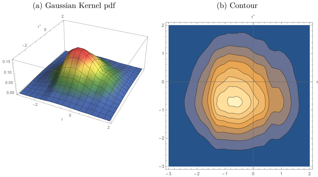
Figure 7: Joint Kernel Density
