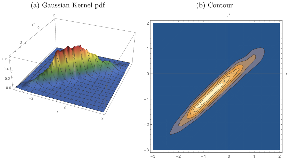
Figure 4: Joint Kernel Density
