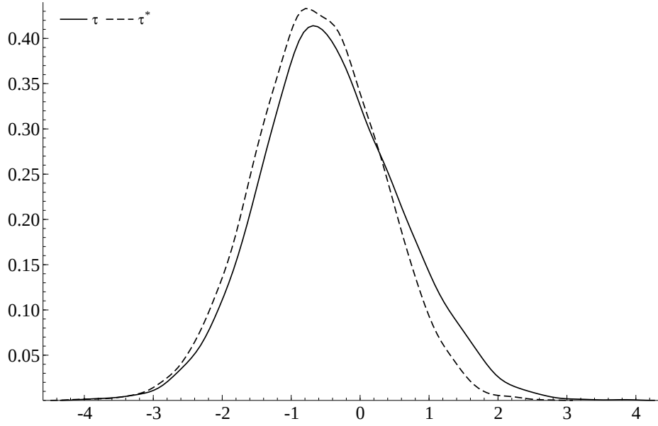
Figure 3: Distribution of the MEB statistic under H_0 : \rho = 1 .
