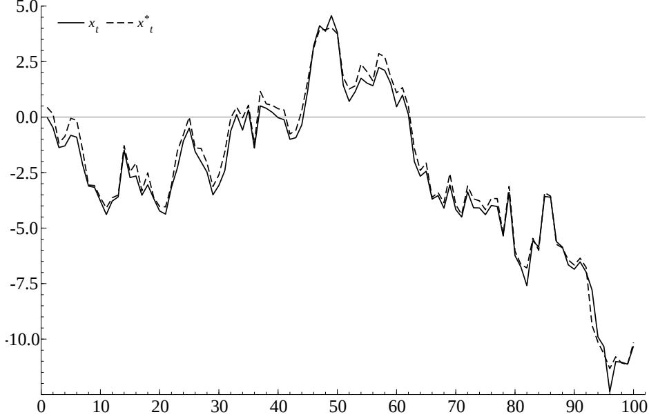
Figure 1: The MEB sample path replication.
