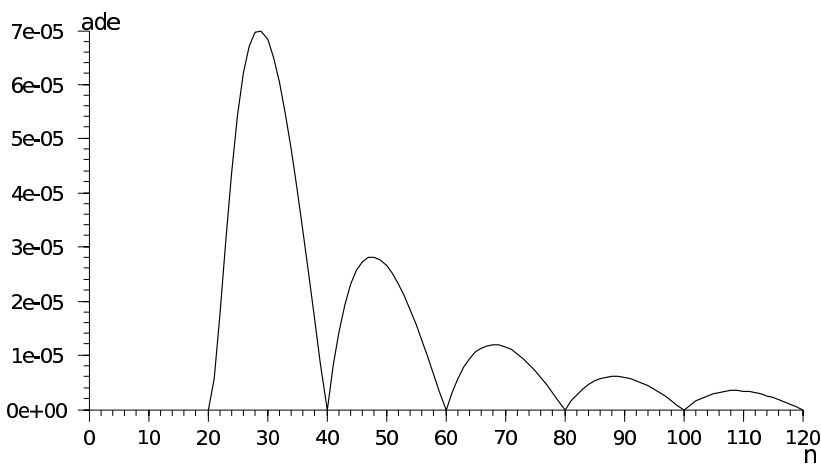
Plot 6. The ade curve when only freeriders arrive.
