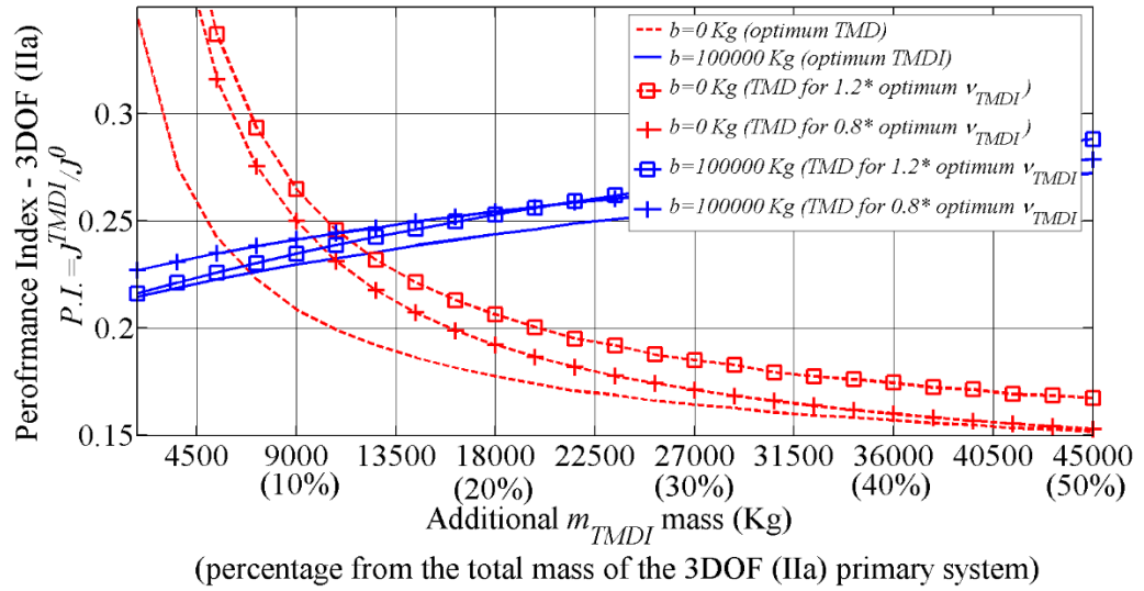
Figure 5.17. Three DOF primary structure - 3DOF (IIa). Performance index versus the additional m_{TMDI} mass for various values of b . Robustness assessment of optimal TMDI on structures with uncertainty in natural frequency.
