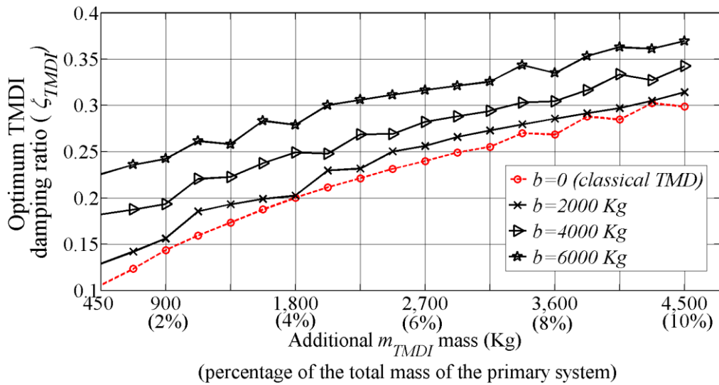
Figure 4.4. Optimum damping ratio as a function of the TMD mass for various values of the inerter constant b to control the fundamental mode of vibration of the 3-DOF primary structure of Table 4.1.
