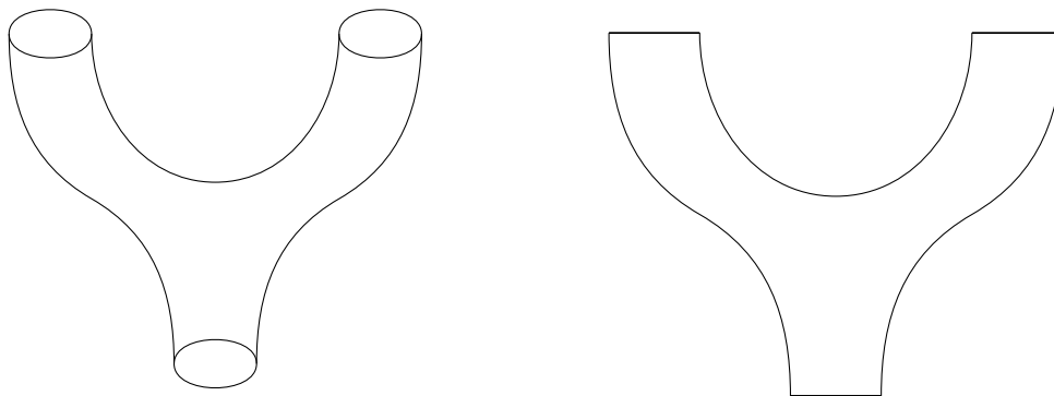
Figure 2: String interactions: splitting of a closed string (left) and an open string (right).
