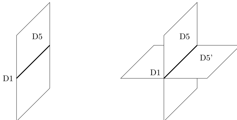
Figure 4: Three-dimensional representation of a D1-D5 system (left) and D1-D5-D5' system (right).
