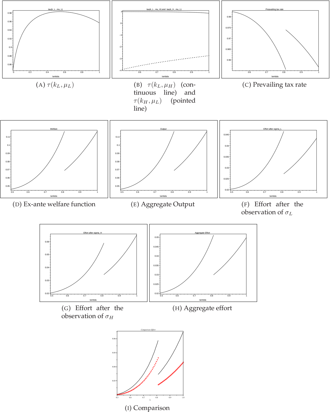
FIGURE 2. Endogenous variables with heterogeneous endowments, for \pi = 0.7, \theta_L = 1, \theta_H = 1.5, a = 8, k_L = 1, k_H = 1.812 .
