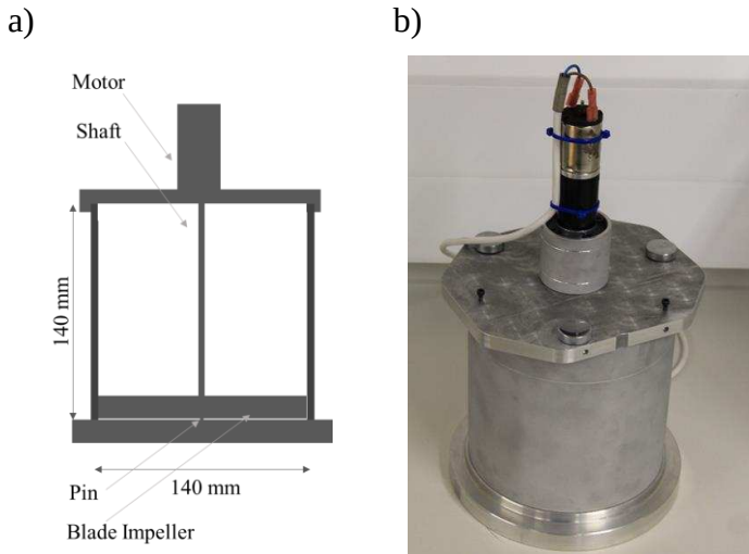
Figure 4. a) Schematic of the mixer with a blade impeller following Cleary & Sinnott (2008), b) A general view of mixer developed for this study.
