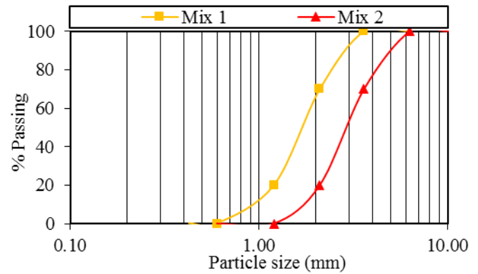
Figure 3. Particle size distribution of two glass ballotini mixes.
