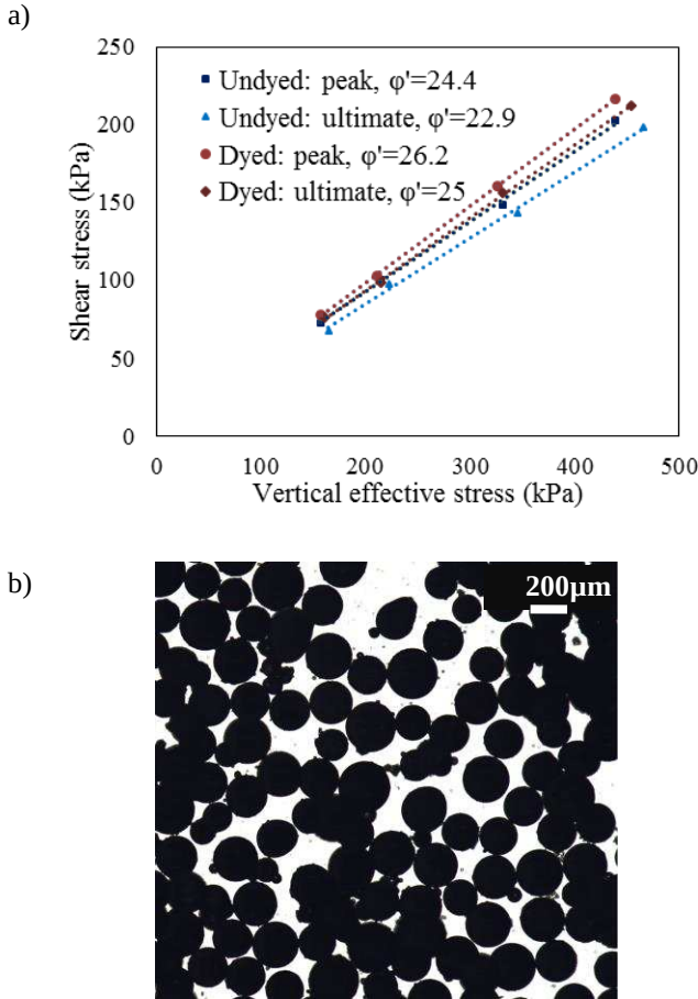
Figure 7. a) Direct shear results for dyed and non-dyed glass ballotini, b) dyed glass ballotini viewed under a microscope.
