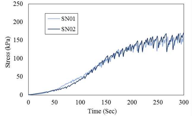
Figure 8. Stress vs. time curves for centrifuge verification tests.
