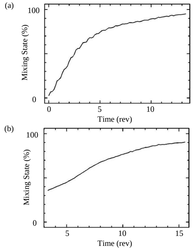
Figure 5. The mixing state for a high shear mixer with a blade impeller as a function of time for: (a) azimuthal and (b) radial mixing from DEM simulations by Cleary and Sinnott (2008).
