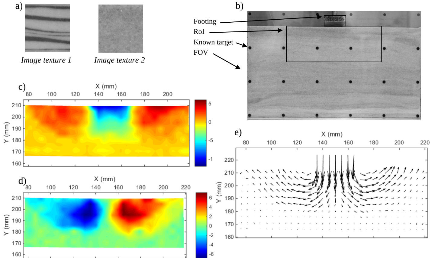
Figure 5. Ballotini-footing interaction, a) Image textures, b) general view, c) vertical displacement, d) horizontal displacement, e) resultant displacement arrows.
