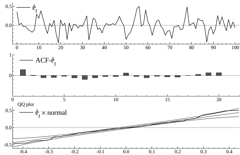
Figure 2.3: SB procedure final selected model plots. The first plot reports the residuals \hat{e}_t time series. The second plot reports the autocorrelation function of \hat{e}_t up to the 20 th lag. The third plot reports the QQ-plot of \hat{e}_t against a standard normal.
