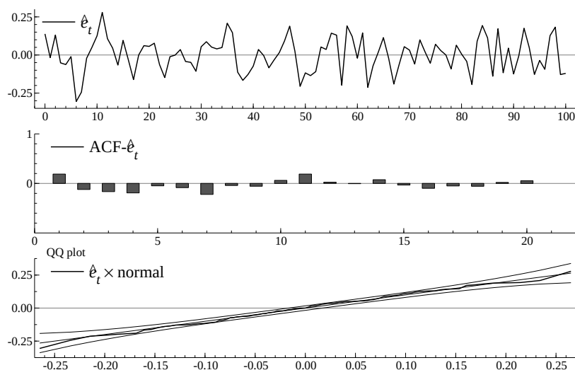
Figure 2.2: US procedure final selected model plots. The first plot reports the residuals \hat{e}_t time series. The second plot reports the autocorrelation function of \hat{e}_t up to the 20 th lag. The third plot reports the QQ-plot of \hat{e}_t against a standard normal.
