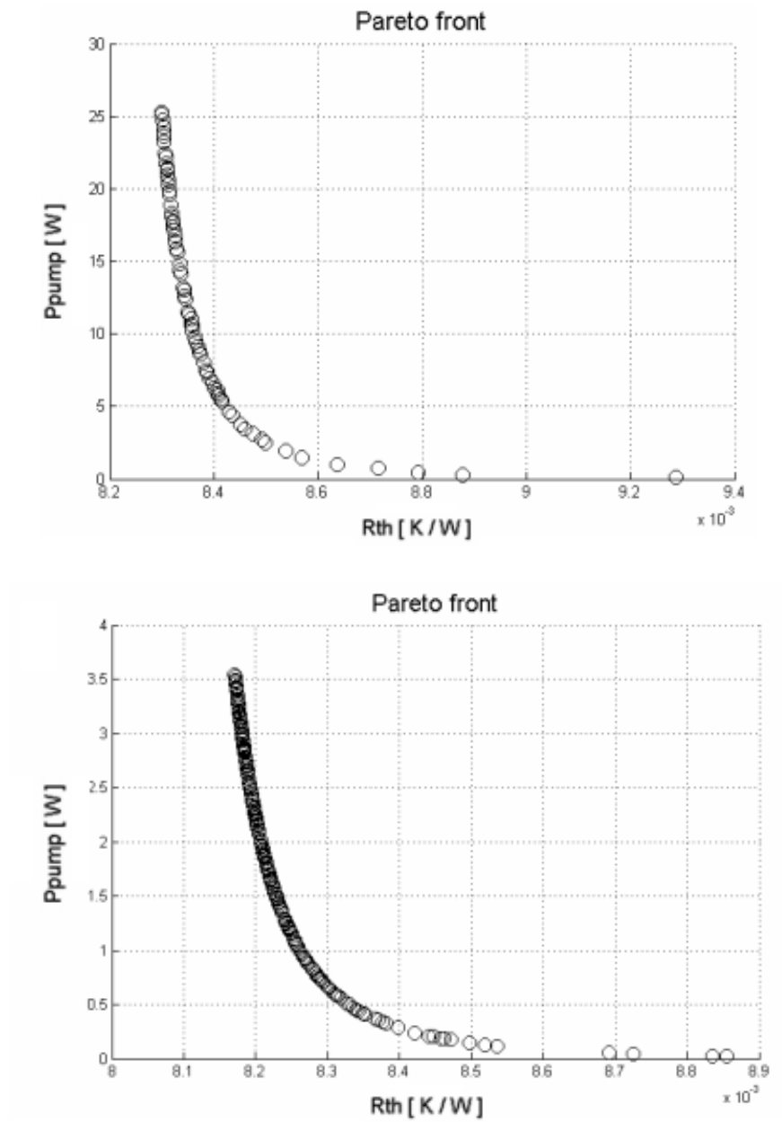
Fig. 6 Pareto front of non dominated solutions (a) for the FW \mu heat sink and (b) for the VW \mu heat sink.
