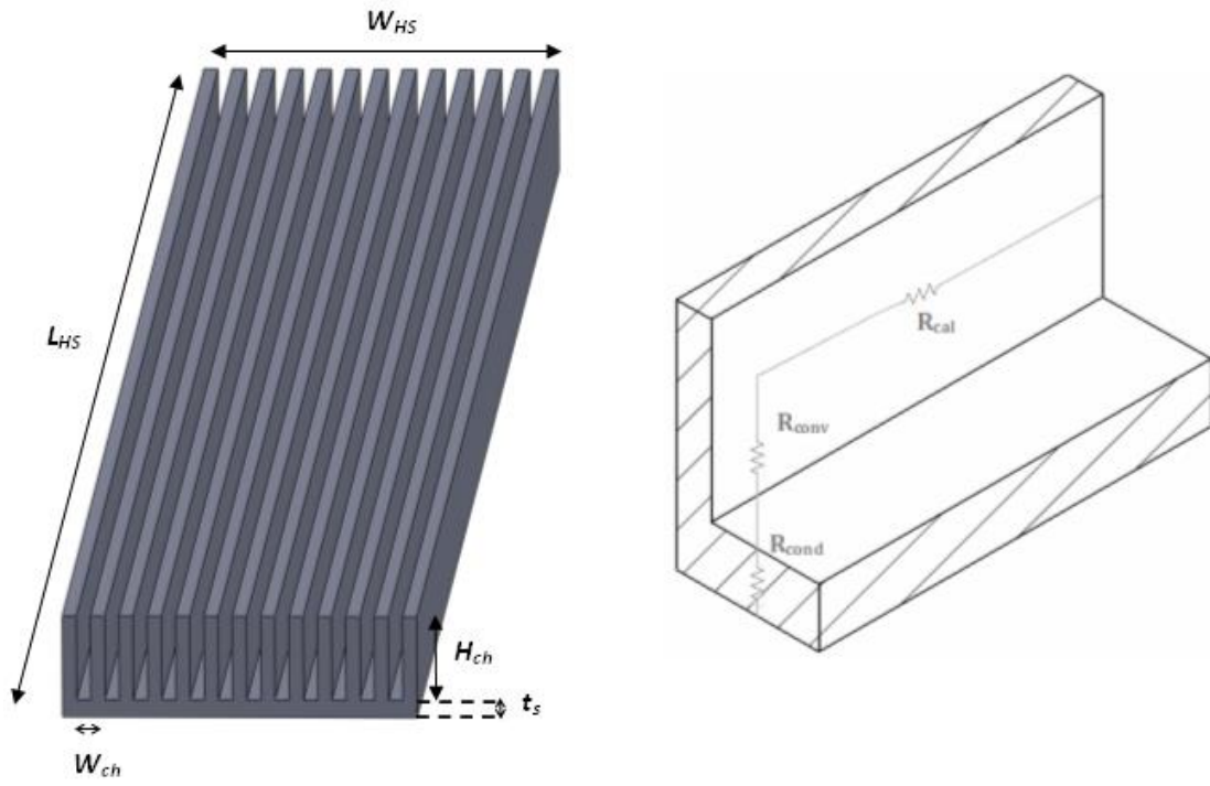
Fig. 2 FWμ heat sink: (a) Layout and (b) equivalent total thermal resistance network.
