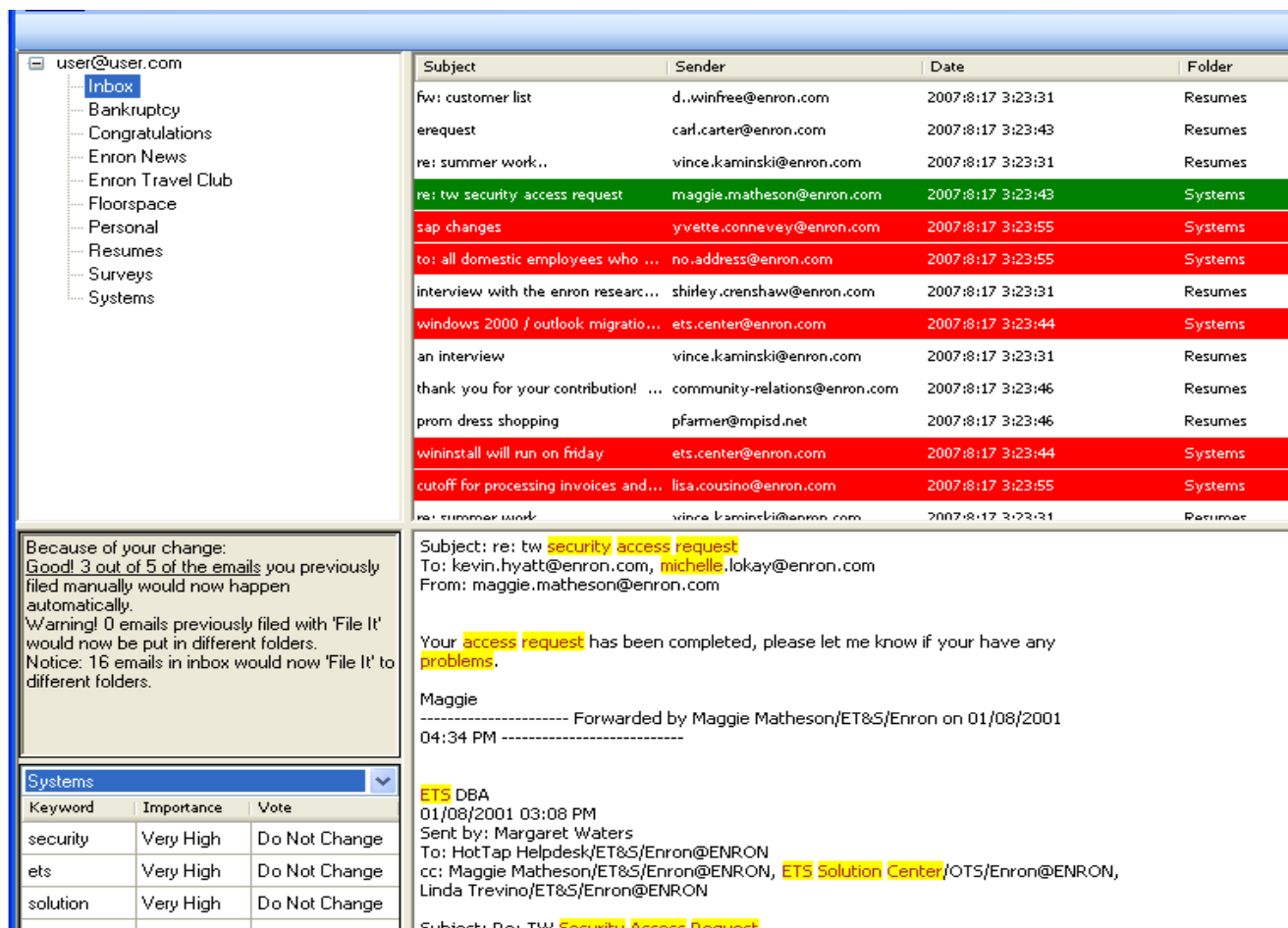
Figure 1. A partial screenshot of the E-mazing email program.
