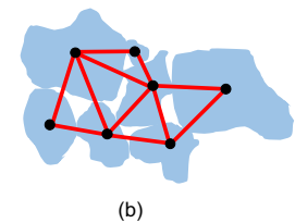
Fig. 7. Schematic diagram illustrating the grain arrangement due to thermal cycling leading to a more compacted fabric (filling of large void) and formation of a new contact network: (a) contact network before thermal cycling; (b) contact network after thermal cycling
