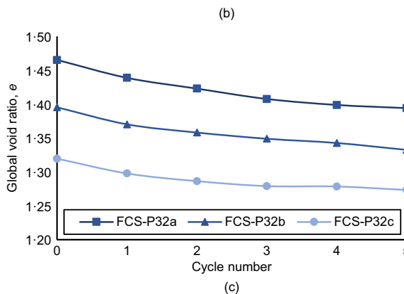
Fig. 6. Void ratio evolution for five thermal cycles using a PMMA container (P32) for: (a) coarse carbonate sand (CCS); (b) silica sand (SS); (c) fine carbonate sand (FCS)
