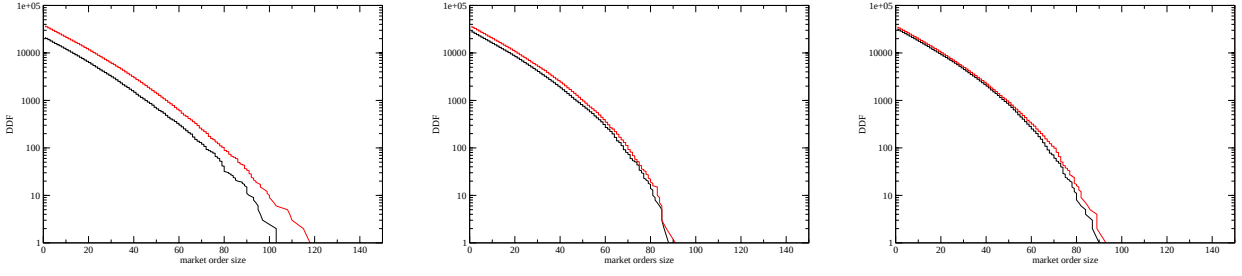
Figure 6: The decumulative distribution function (not normalized) of market order size for buy (black) and sell (red) orders with noise trading (left), noise trading and fundamentalism (centre), and noise trading, fundamentalism and chartism (right). The value of the parameters are the same as in Figure 5.
