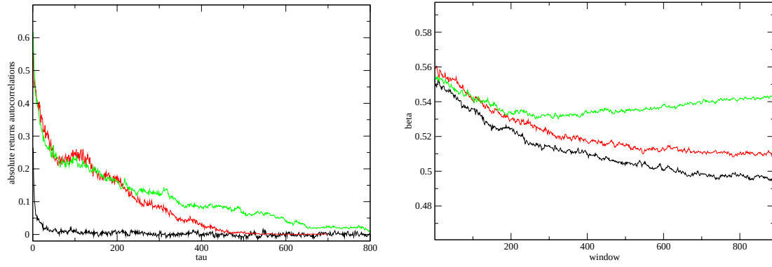
Figure 5: (Left) Volatility autocorrelation decays for noise trading (black, \sigma_1 = \sigma_2 = 0.00 ), noise trading and fundamentalism (red, \sigma_1 = 10.00 , \sigma_2 = 0.00 ) noise trading fundamentalism and chartism (green, \sigma_1 = 10.00 , \sigma_2 = 1.20 ). (Right) The modified R/S exponent for absolute returns on the left side in terms of the time window. We here represent the exponent \beta_n for several trading weights and filter the short term memory for a number of time steps q = 20 (cf. Eq. (14)).
