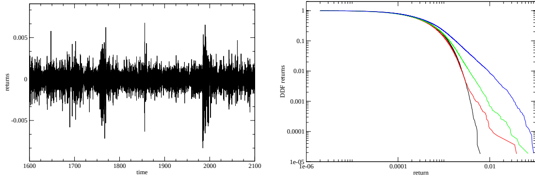
Figure 3: (Left) Return time series with noise trader, fundamentalist and chartist ( \sigma_1 = 10.00 , \sigma_2 = 1.20 ) components all present. (Right) The decumulative distribution function of the absolute returns with \sigma_1 = 10.00 and \sigma_2 = 0.00 (black), \sigma_2 = 1.20 (red), \sigma_2 = 2.00 (green), \sigma_2 = 2.80 (blue).
