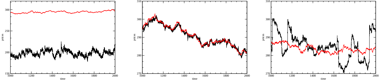
Figure 2: Price (black) and fundamental value (red) with only noise trading (left, \sigma_1 = 0.00, \sigma_2 = 0.00 ), noise trading and fundamentalism (center, \sigma_1 = 10.00, \sigma_2 = 0.00 ) and noise trading, fundamentalism and chartism (right, \sigma_1 = 10.00, \sigma_2 = 1.20 ).
