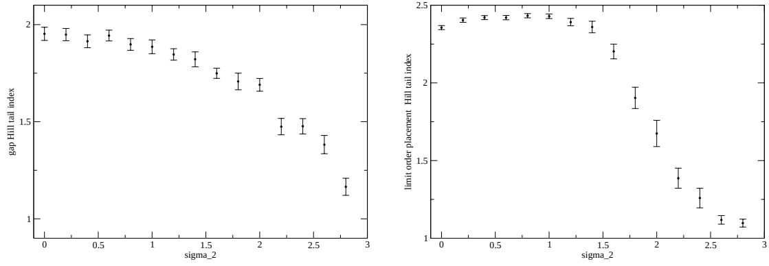
Figure 8: (Left) Hill exponent of the first gap distribution for \sigma_1 = 10.00 and different values of \sigma_2 . (Right) Hill exponent of the order placement distribution for \sigma_1 = 10.00 and different values of \sigma_2 .
