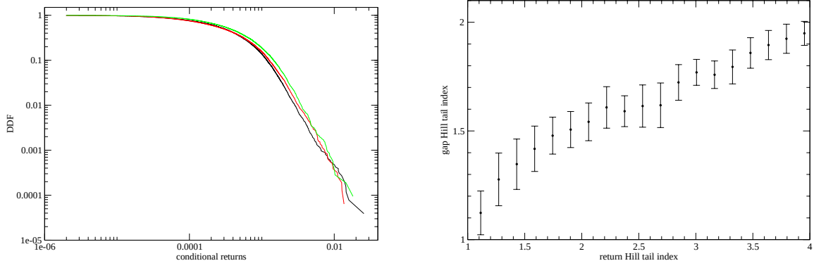
Figure 11: (Left) Conditional returns for different trading volume: size < 15 (black), 15 < \text{size} < 30 (red), size > 30 (green), for \sigma_1 = 10 and \sigma_2 = 2.0 . (Right) The tail index of the first gaps versus the tail index of returns for \sigma_1 = 10 and different values of \sigma_2 .
