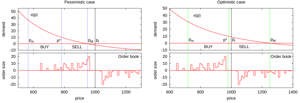
Figure 9: (Left) The role of the CARA demand function (5) in the order placement decision when p_M = \hat{p}_{t+\tau^i}^i < p_t and for a given snapshot of the book. (Right) The role of the CARA demand function (5) in the order placement decision when p_M = \hat{p}_{t+\tau^i}^i > p_t and for a given snapshot of the book. The figures at the bottom show a typical pattern of the limit order book at a given time in a simulation. Buy orders placed in the book are represented as positive volume, while sell orders placed in the book are represented as negative volume. The top figures are particular instances of Figure 1. The intersections determine the three different price levels p_m , p^* and p_M for the case of optimistic trader ( p_M > p_t ) (right) and pessimistic trader ( p_M < p_t ) (left).
