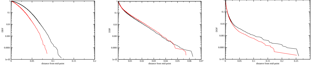
Figure 7: The decumulative distribution function of limit order placement distance from the midpoint for buy (black) and sell (red) orders with noise trading (left), noise trading and fundamentalism (centre), and noise trading, fundamentalism and chartism (right). The value of the parameters are the same as in Figure 5.
