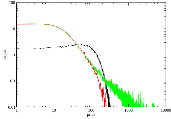
Figure 10: The book shape (on log-log scale) with noise trading (black), noise trading and fundamentalism (red), noise trading fundamentalism and chartism (green). The book has a more realistic shape with the depth higher toward the best price and fat tails appearing as the chartist component \sigma_2 is activated. The value of the parameters are the same as in Figure 5.
