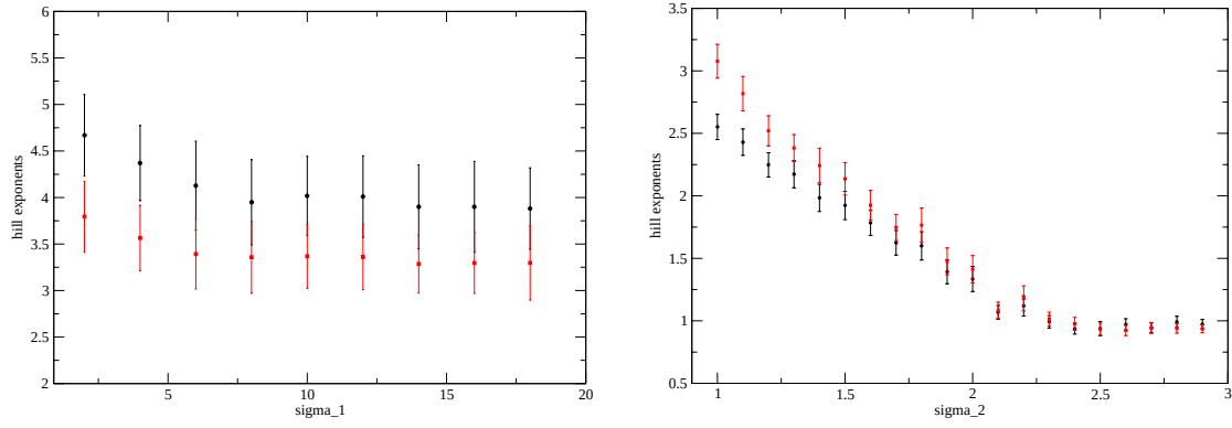
Figure 4: Hill exponents of the left (black) and right (red) tails of the returns distribution as a function of \sigma_1 with \sigma_2 = 0.00 (left) and as a function of \sigma_2 with \sigma_1 = 10.00 (right). Vertical spreads depicts the error bars for the Hill exponent which are evaluated across 100 repetitions of the simulations with different random seeds.
