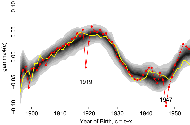
Fig. 15. Cohort effect \gamma^{(4)}(c) for the stochastic mortality model (equation (4)) by using unadjusted (—●—) and adjusted (—, —) exposures data: —, 90% credibility interval (bounded by the 5–95% quantiles of the posterior distribution) for \gamma^{(4)}(c) ; —, a typical realization of \gamma^{(4)}(c) from the posterior distribution
