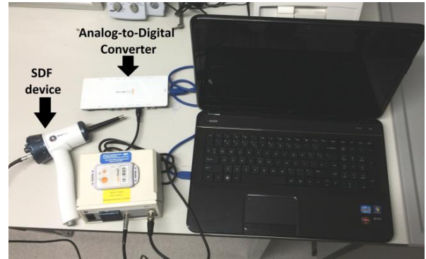
Fig. 2 The setup of the experiment includes the SDF imaging device (left, the ADC (up-left) and the laptop (right) running the AVA 3.2 software
