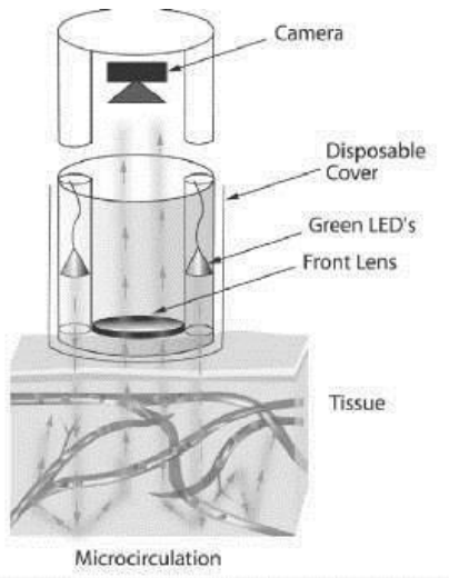
Fig. 1 Sidestream Dark Field imaging configuration [10]
