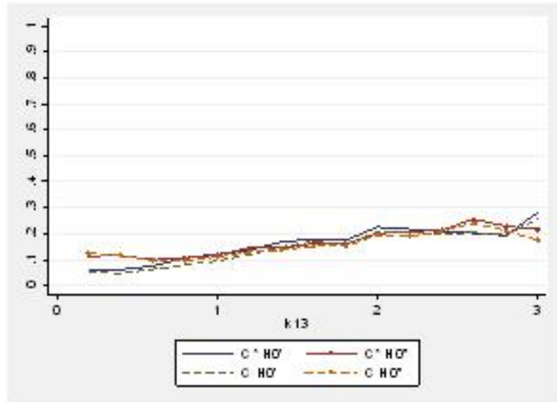
Figure 8: BEE with arbitrary values of \kappa_{13} - C(\alpha) tests
