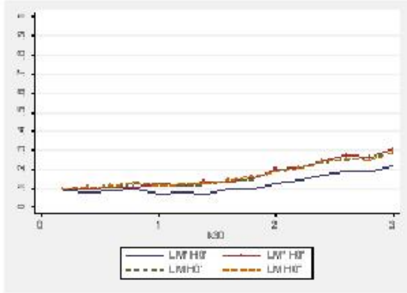
Figure 9: BEE with arbitrary values of \kappa_{30} - LM tests
