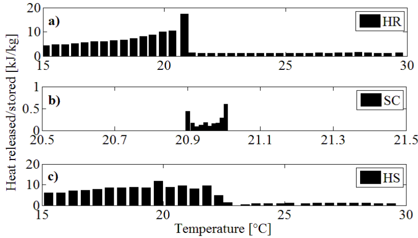
Figure 2. Experimental results for the heat storage in the given temperature intervals for the RT21 PCM ( m=41 g). a) Heat Released (HR) upon sample freezing, b) degree of SubCooling (SC) upon sample freezing, and c) Heat Stored (HS) upon sample melting.
