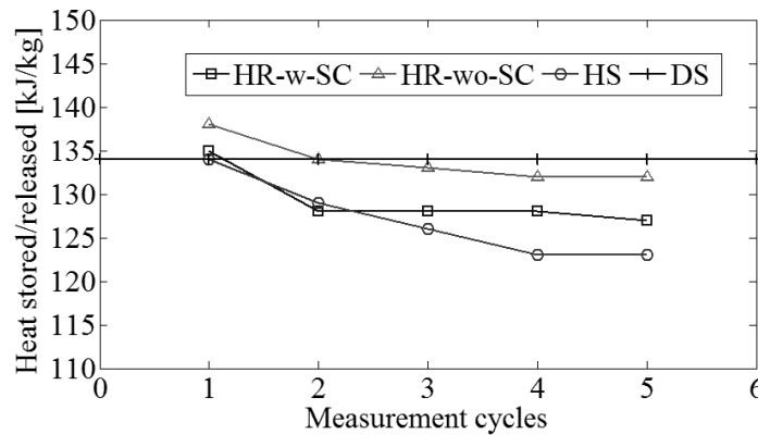
Figure 3. Experimental results for the heat storage of the RT21 sample ( m=41 g) evaluated in the 15 – 30 °C temperature range (HR SC – Heat Released with taking SubCooling effect into the account, HR no SC – Heat Released without taking SubCooling effect into the account, HS – Heat Stored, DS – heat Data Sheet value).
