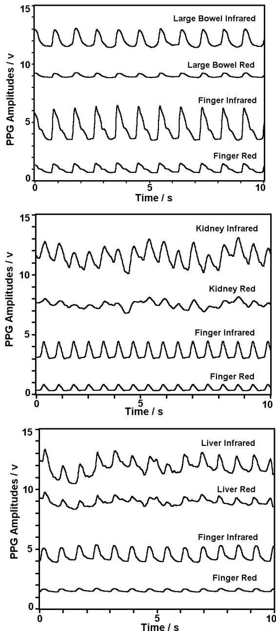
Figure 3: AC PPG traces on laptop from simultaneous measurements at various abdominal organs (bowel, kidney, and liver) and the finger.
