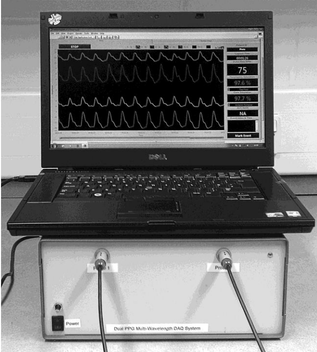
Fig.2: Photo of the fontanelle/foot PPG system
