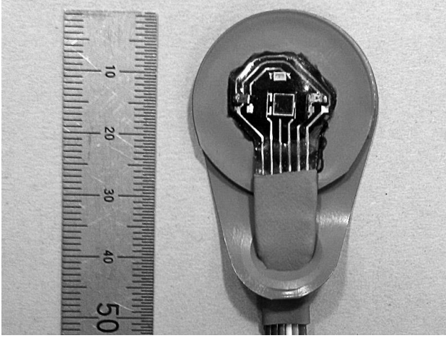
Fig. 1: Custom PPG fontanelle sensor.
