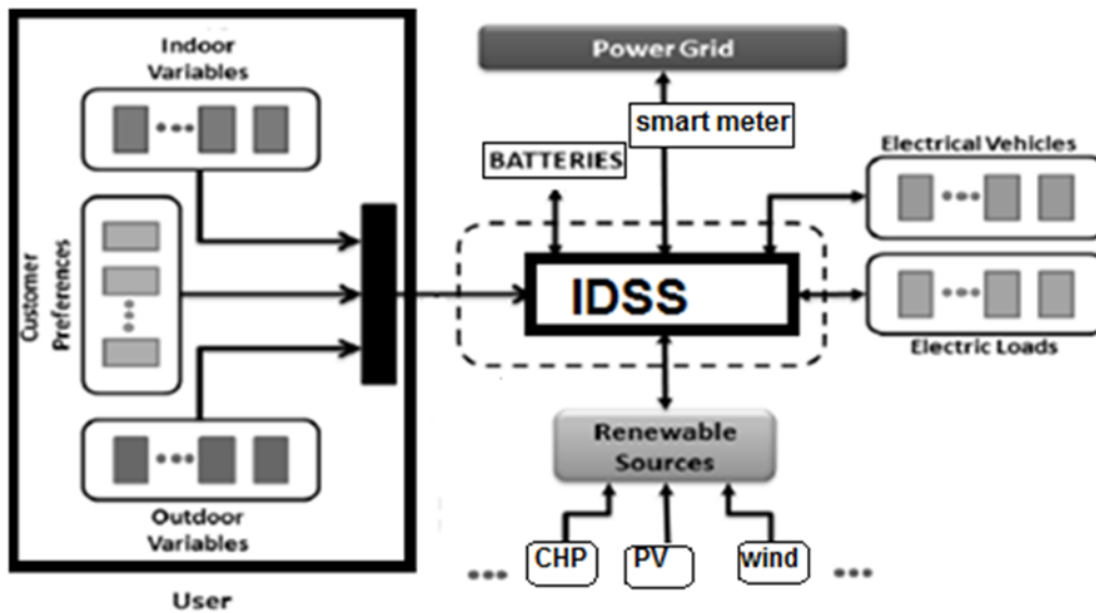
Figure 4.2 Structure of Home Energy Management System
