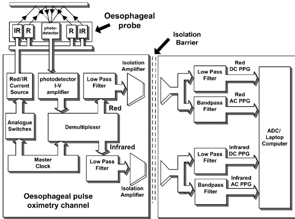
Figure 9. Oesophageal pulse oximeter processing system.
