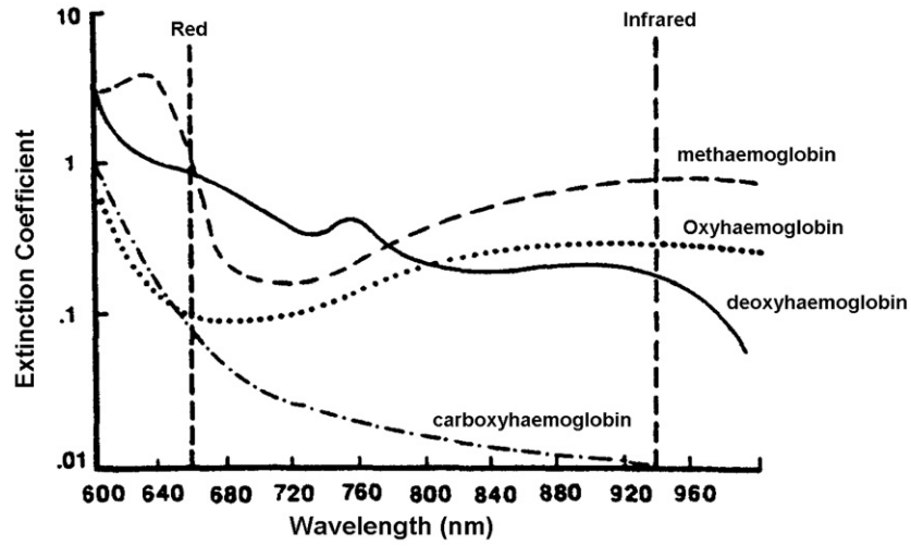
Figure 2. Extinction coefficients ( \text{Lmmol}^{-1} \text{cm}^{-1} ) of the four most common haemoglobin species; oxyhaemoglobin ( \text{HbO}_2 ), deoxyhaemoglobin (Hb), carboxyhaemoglobin (COHb) and methemoglobin (MetHb) at the wavelengths of interest in pulse oximetry.
