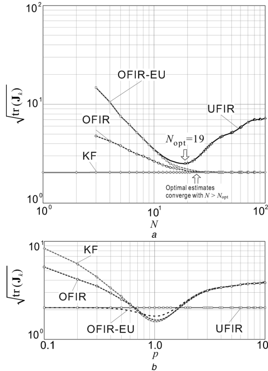
Fig. 7 RMSEs \sqrt{\text{tr} \mathbf{J}_k} in the estimates of the two-state harmonic model
