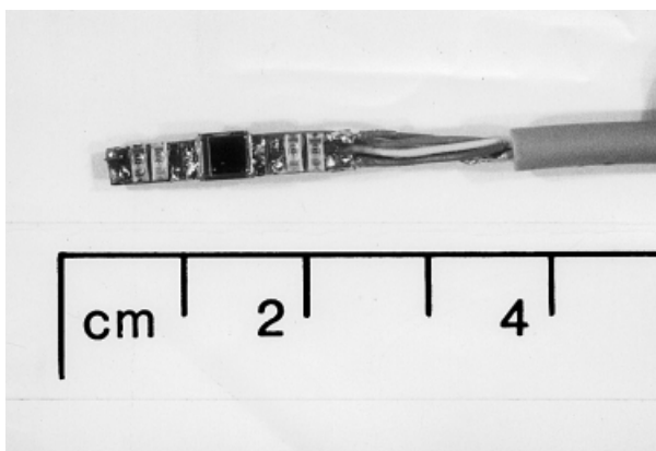
Figure 1 Reflectance visceral photoplethysmographic probe used to measure splanchnic oxygen saturation.
