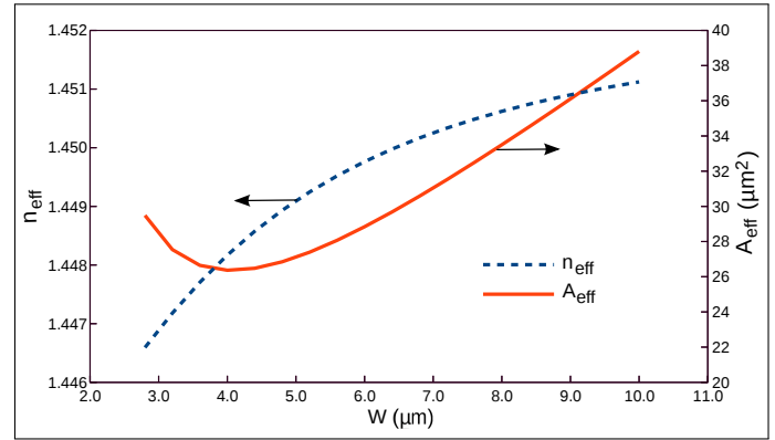
Fig. 6. Variations of the n_{eff} and A_{eff} of the H_{11}^Y mode with the guide width, W .
