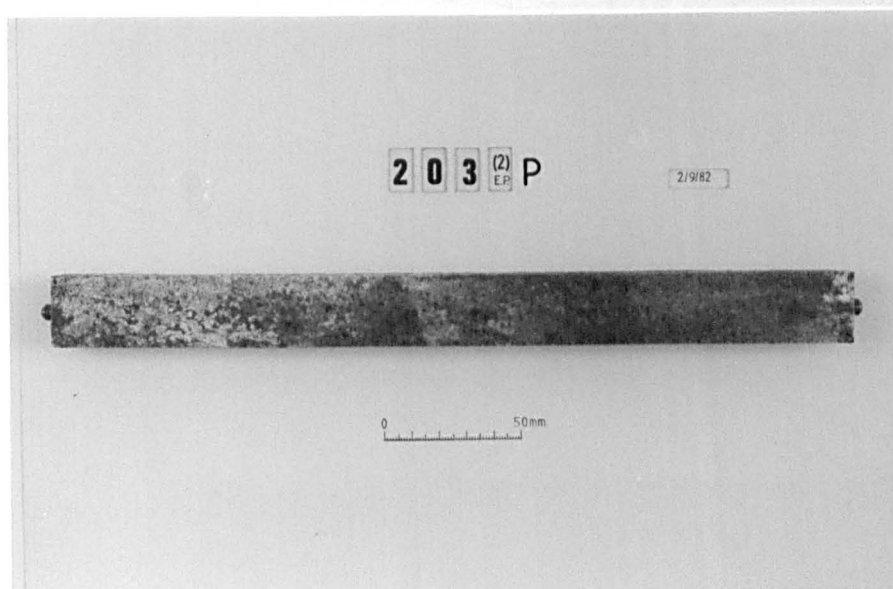
Plate 6.12 Mix Ref. 2032P, showing the surface condition of a typical mortar bar subsequent to the expansion measurement taken at age 6 months.
