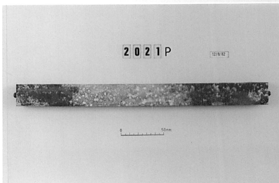
Plate 6.4 Mix Ref. 2021P, showing the surface condition of a typical mortar bar subsequent to the expansion measurement taken at age 6 months.
