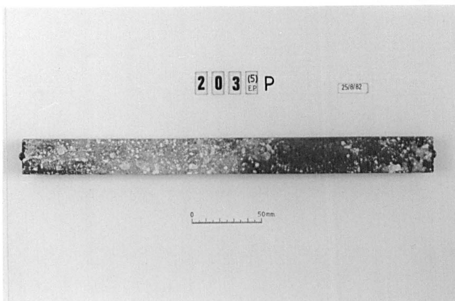
Plate 6.13 Mix Ref. 2035P, showing the surface condition of a typical mortar bar subsequent to the expansion measurement taken at age 6 months.
