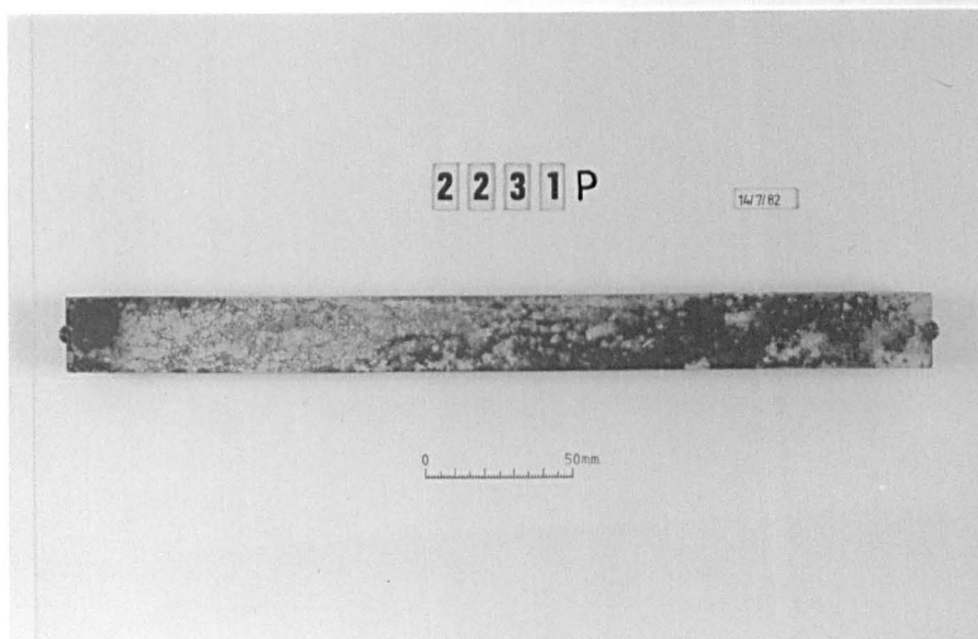
Plate 6.8 Mix Ref. 2231P, showing the surface condition of a typical mortar bar subsequent to the expansion measurement taken at age 6 months.
