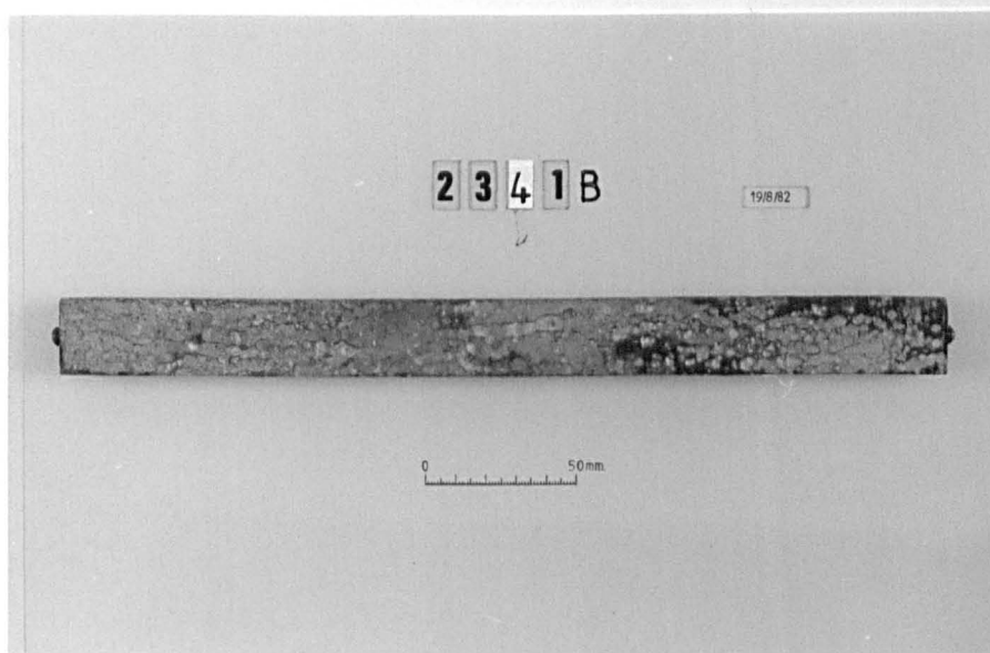
Plate 6.18 Mix Ref. 2341B, showing the surface condition of a typical mortar bar subsequent to the expansion measurement taken at age 6 months.
