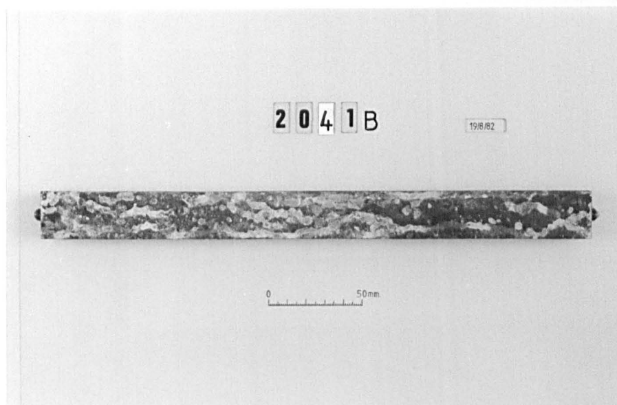
Plate 6.17 Mix Ref. 2041B, showing the surface condition of a typical mortar bar subsequent to the expansion measurement taken at age 6 months.
