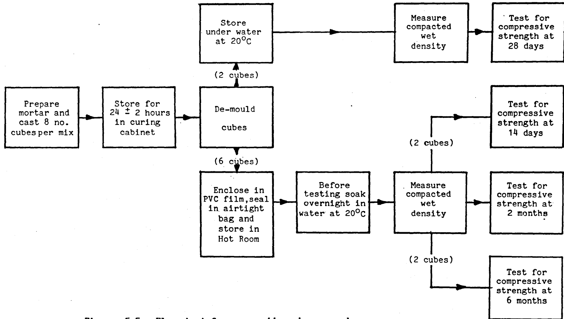
Figure 5.5 Flow chart for preparation, storage and testing of 2" cubes
