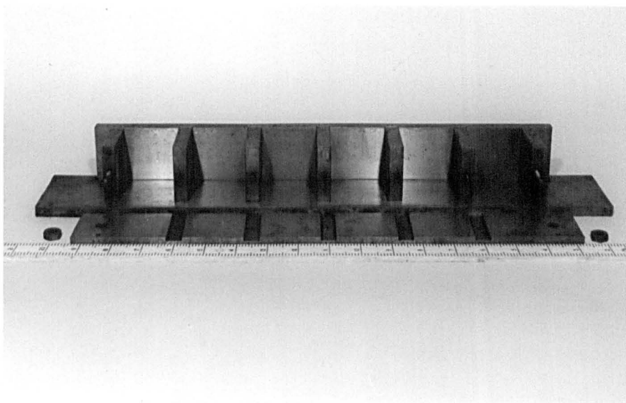
Plate 5.9 Gang mould capable of making six cube specimens (2").
