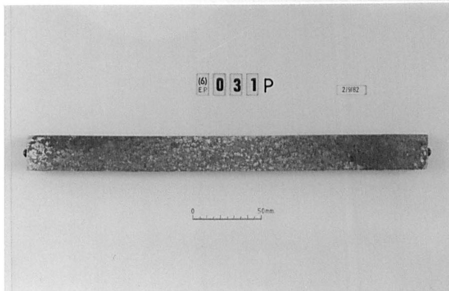
Plate 6.16 Mix Ref. 6031P, showing the surface condition of a typical mortar bar subsequent to the expansion measurement taken at age 6 months.
