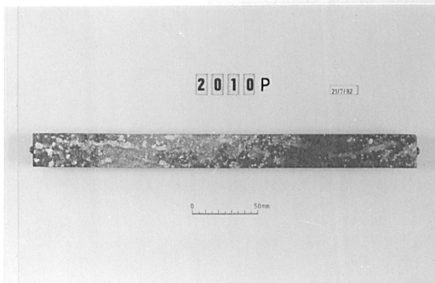
Plate 6.2 Mix Ref. 2010P, showing the surface condition of a typical mortar bar subsequent to the expansion measurement taken at age 6 months.
