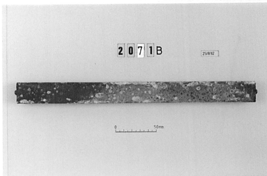
Plate 6.19 Mix Ref. 2071B, showing the surface condition of a typical mortar bar subsequent to the expansion measurement taken at age 6 months.
