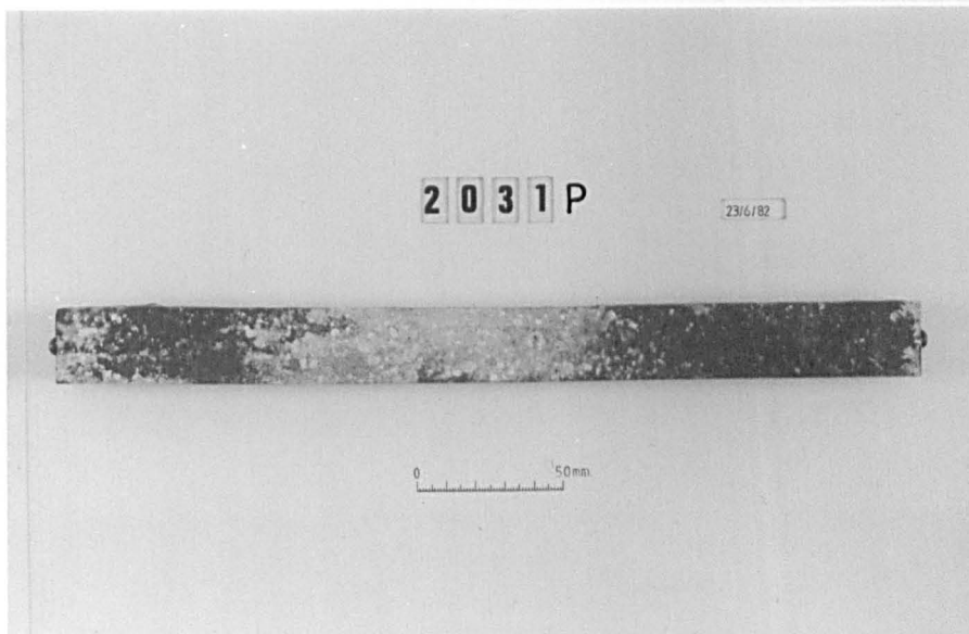
Plate 6.6 Mix Ref. 2031P, showing the surface condition of a typical mortar bar subsequent to the expansion measurement taken at age 6 months.
