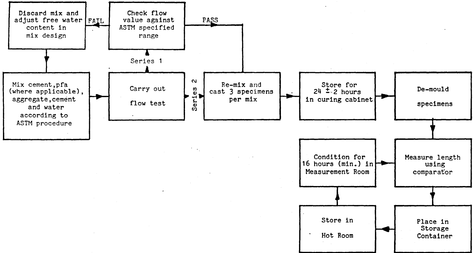
Figure 5.4 Flow chart for preparation, storage and measurement of mortar bars, Series 1 & 2
