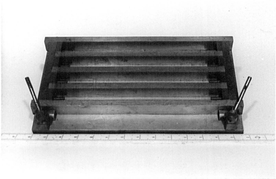
Plate 5.5 Gang mould capable of making four mortar bar specimens with encastre gauge studs.
