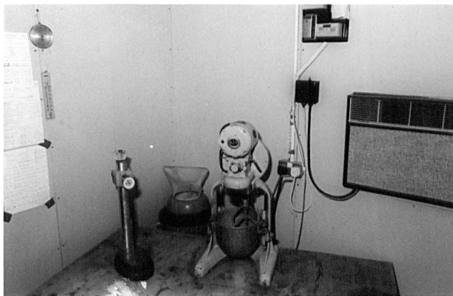
Plate 5.4 Inside view of moulding/measurement room, showing Hobart mixer, length comparator, heater/refridgeration unit and humidifier.
