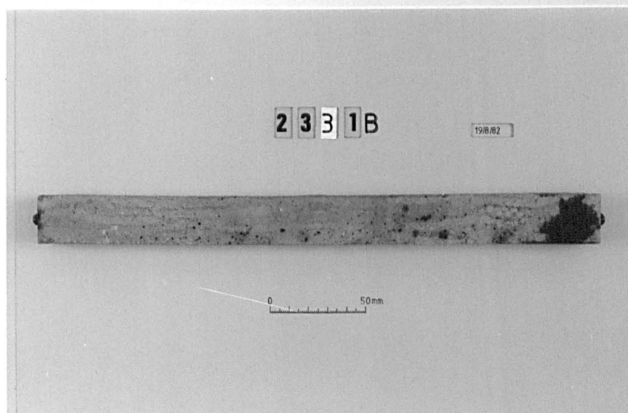
Plate 6.22 Mix Ref. 2331B, showing the surface condition of a typical mortar bar subsequent to the expansion measurement taken at age 6 months.
