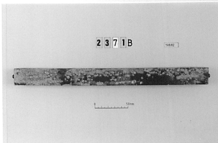
Plate 6.20 Mix Ref. 2371B, showing the surface condition of a typical mortar bar subsequent to the expansion measurement taken at age 6 months.
