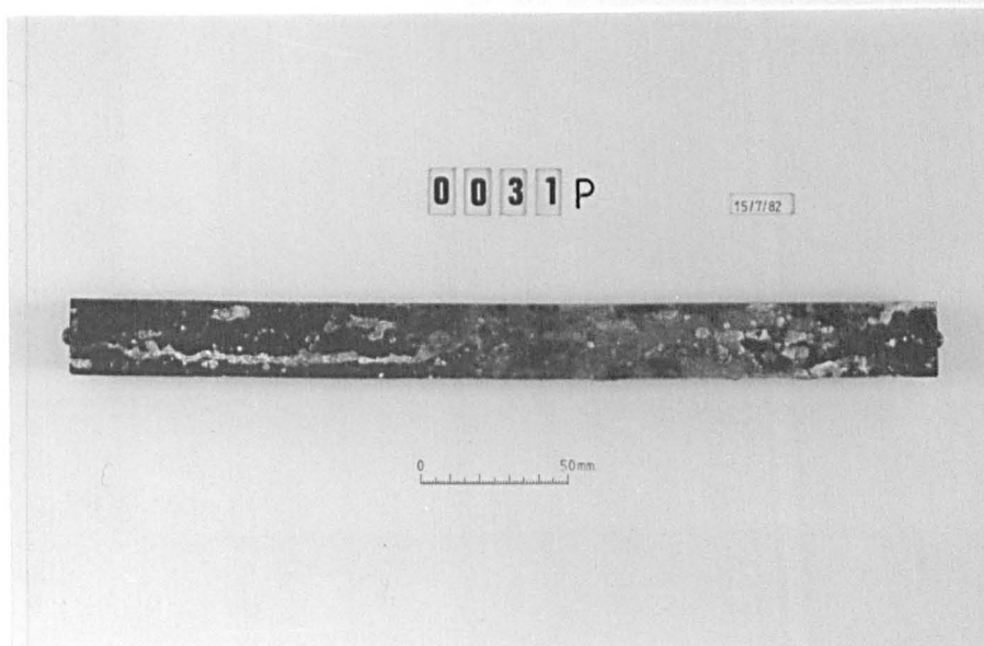
Plate 6.10 Mix Ref. 0031P, showing the surface condition of a typical mortar bar subsequent to the expansion measurement taken at age 6 months.
