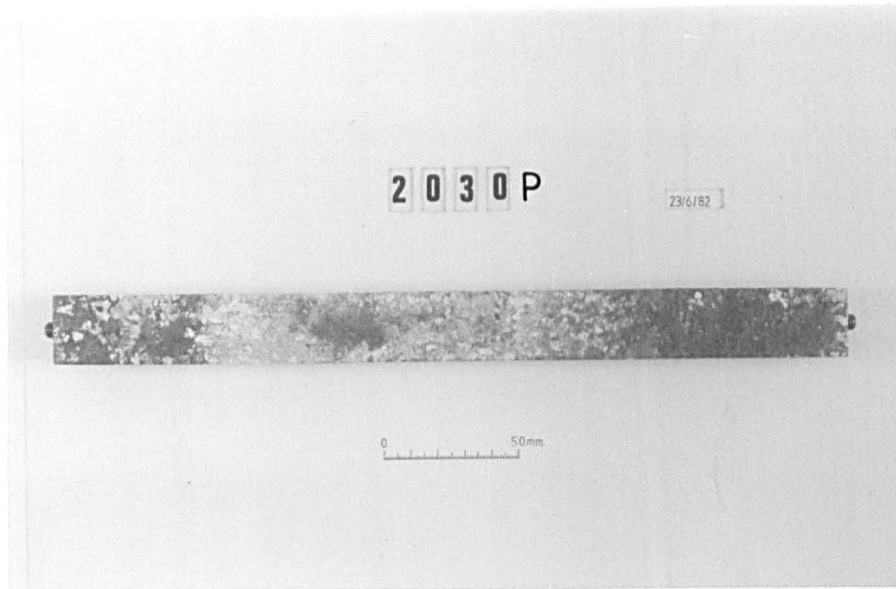
Plate 6.5 Mix Ref. 2030P, showing the surface condition of a typical mortar bar subsequent to the expansion measurement taken at age 6 months.
