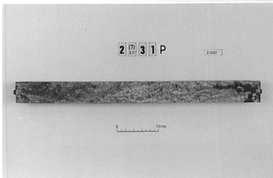
Plate 6.14 Mix Ref. 2731P, showing the surface condition of a typical mortar bar subsequent to the expansion measurement taken at age 6 months.
