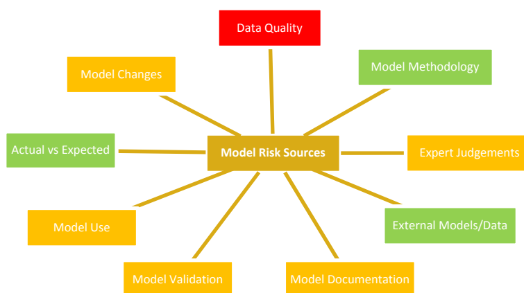
Figure 2.3: Diagrammatic presentation of qualitative model risk assessment
