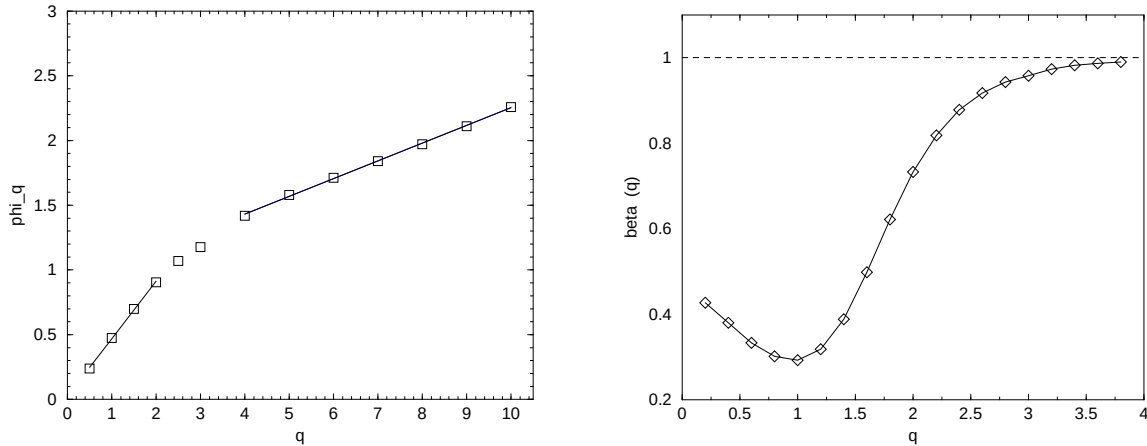
FIGURE 1. Exponent \phi_q versus q (left). The slope of the two regions are 0.47 at q < 3 and 0.14 at q > 3 . Scaling exponent \beta(q) as a function of q (right). Anomalous scaling with \beta(q) < 1 is shown.
