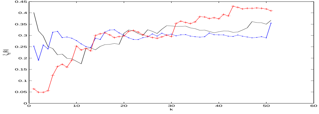
Figure 5.2. Hill's plot. (-) depicts the path of tail index estimates of DJBC Index, (-) of DJSI Index and (+-) of Ftse100.
