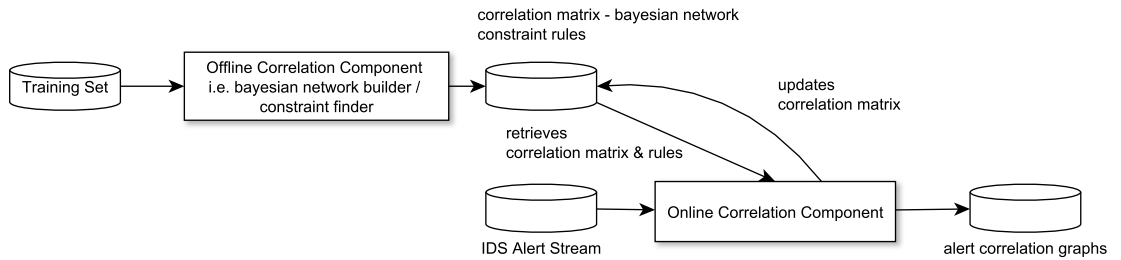
Figure 3.3: Architecture of the Posterior Correlation Model.
