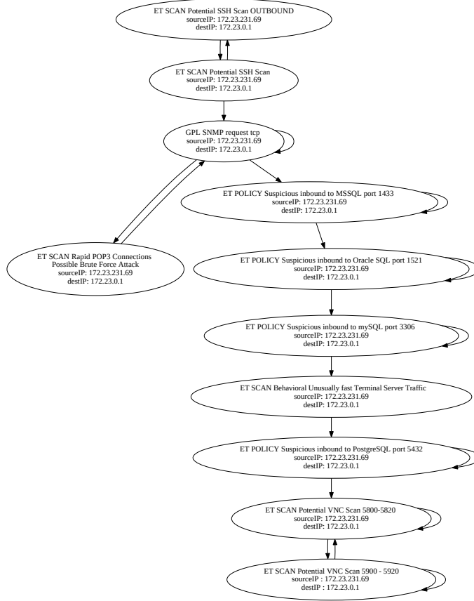
Figure 5.9: Centroid of C_5
