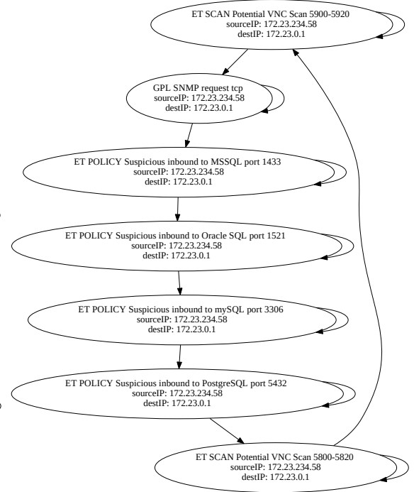
Figure 5.10: Centroid of C_6
