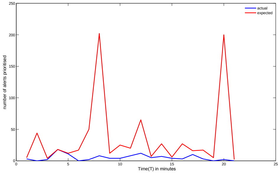
Figure 4.8: Performance of Attack Duration Rate Metric on DARPA Dataset showing Actual vs Expected Priority Distribution
