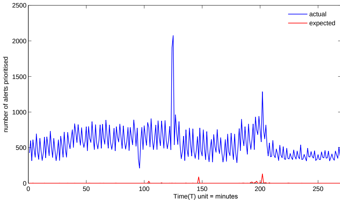
Figure 4.12: Prioritisation Results using Outgoing rate Metric on the Northrop Grumman II Internal Attack Dataset
