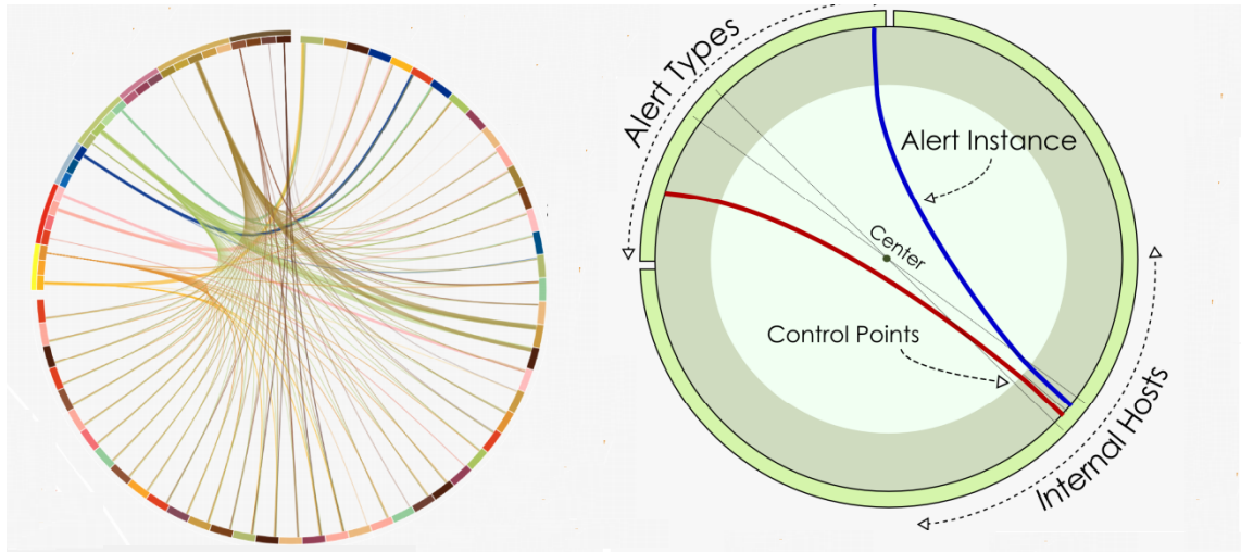
Figure 2.14: Avisa - A radial network visualisation proposed by Shiravi et al. [152]
