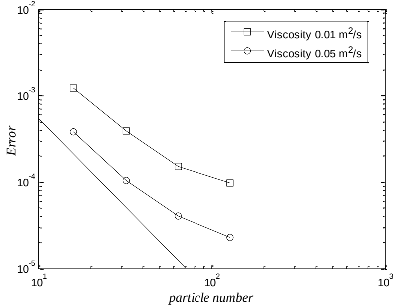
Figure 7.9: Errors for different particle numbers of 16, 32, 64 and 128 in a wave length for the viscosities of 0.01m 2 /s and 0.05m 2 /s. The solid line indicates the second order convergence.
