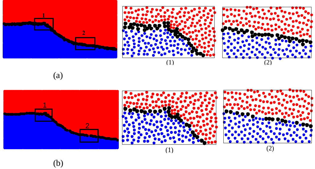
Figure 4.1: Examples of interface identifications when applying improper value of \gamma . (a) shows inner particles close to the interface are over-identified with \gamma = 0.1 and (b) shows some interface particles are under-identified with \gamma = 0.5 . (density ratio: 1:1000)
