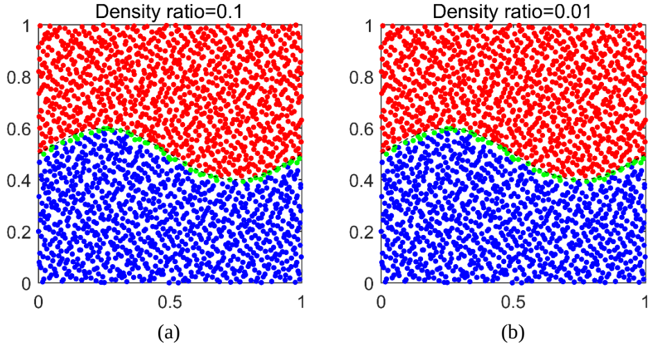
Figure 4.7: Interface particles (green nodes) identification by ADG technique on density ratios of 0.1 with the densities of blue and red dots of 10 and 1 respectively in (a) and 0.01 with the densities of blue and red dots of 100 and 1 respectively in (b).
