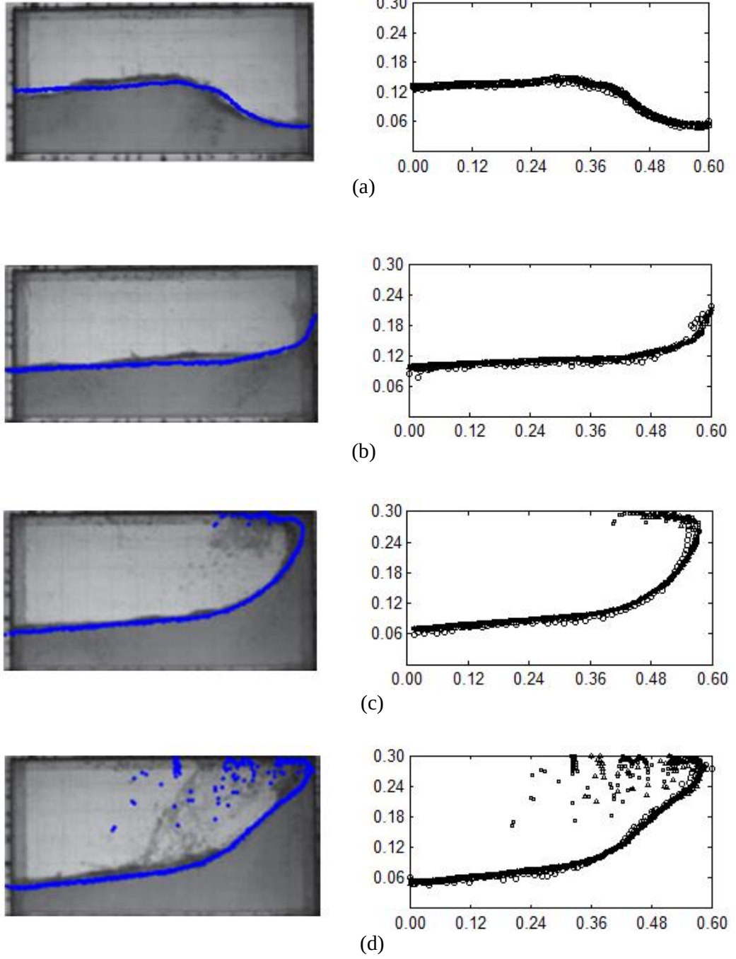
Figure 6.16: Comparison of water-air interface profiles at t=1.43s , 1.56s , 1.69s and 1.82s from (a) to (d). Left column gives experiment photos compared with the simulation of dx = 0.004m . Right column gives MLPG_R results with dx = 0.012m , 0.006m and 0.004m (snapshots in the shape of circle, rectangle and square respectively).
