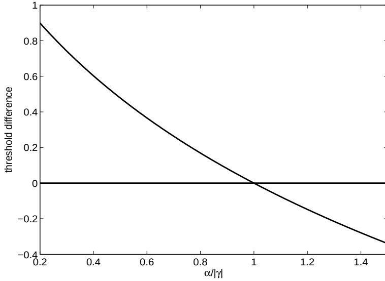
Figure 2: p_{id}^* - \tilde{p}_i^* .
