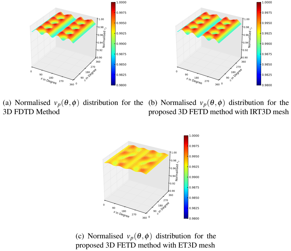
Fig. 11.11 Side by side comparison of normalised v_p of the 3D FDTD and the proposed 3D FETD scheme with the IRT3D and the ET3D meshes at 10/\lambda resolution
