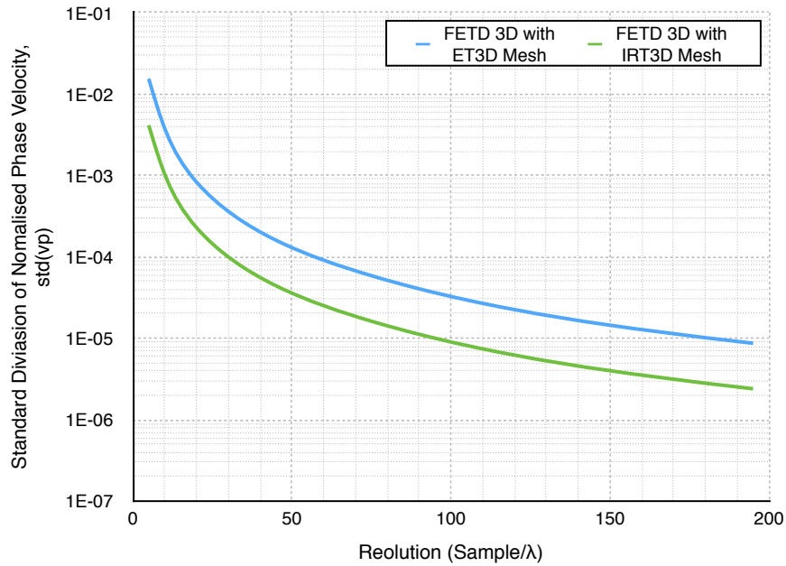
(b) Comparison of the standard deviation of normalised v_p for ET3D and IRT3D meshes
