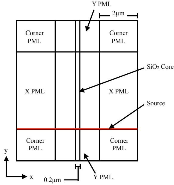
Fig. 6.3 Schematic diagram of the planar waveguide setup
