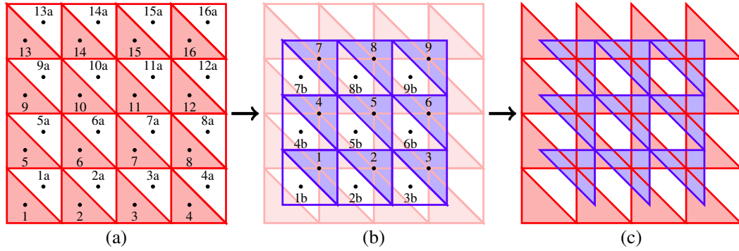
Fig. 3.1 (a) The generating the linear mesh by dividing a square grid by diagonal line, (b) Generating the auxiliary mesh by connecting the centroids of the main mesh, (c) Discarding the unwanted elements from both meshes
