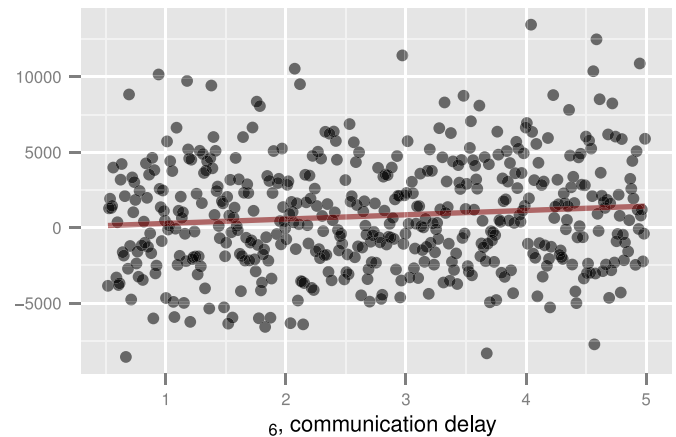
Fig. 12. Residual and component plot for communication delay effects, \hat{\beta}_{6v} , with the fitted trend shown in red. (For interpretation of the references to color in this figure legend, the reader is referred to the web version of this article.)
