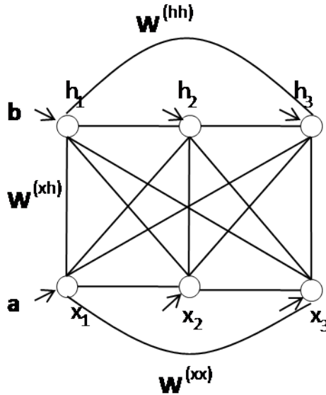
Figure 2.2: A Boltzmann machine.
