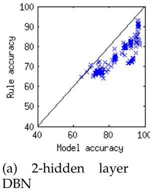
Figure 4.6: Comparison between the test-set accuracies of DBNs (model accuracy) and extracted rules using rule-based early stopping.
