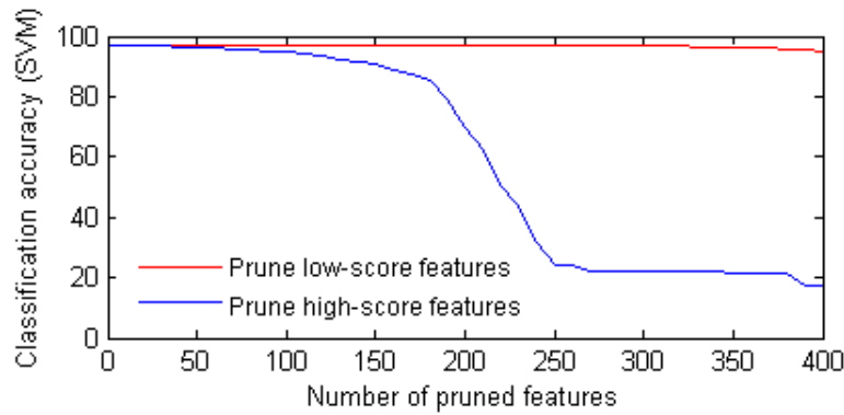
Figure 5.5: Classification accuracy of a pruned RBM, starting with 500 hidden units, on 10,000 MNIST test samples. The red and blue lines represent the accuracy following pruning of low-scoring and high-scoring feature detectors respectively.
