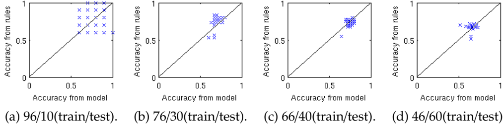
Figure 4.4: Classification performances of DBNs compared with extracted rules on the DNA promoter dataset.
