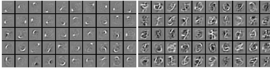
(a) Feature detectors with high scores. (b) Feature detectors with low scores.
