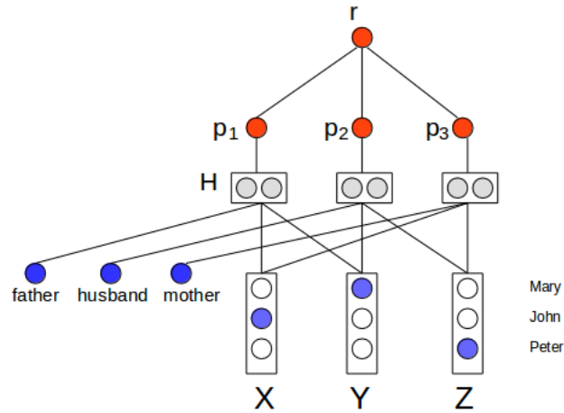
Figure 7.1: Proposed deep relational model.
