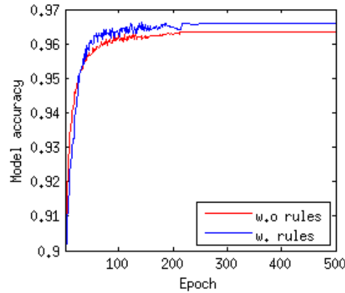
Figure 4.10: Performance of modular DBNs with and without encoded rules.
