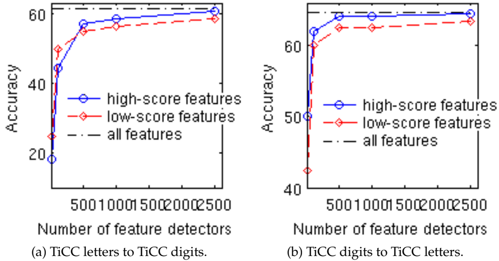
Figure 5.8: Self-taught learning using RBMs where only a subset of features have been transferred.
