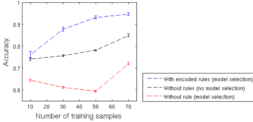
Figure 4.9: Test set classification performance of 2-layer standard DBN (red and black lines, with and without model selection), and 2-layer DBN encoded with prior knowledge from the DNA promoter background theory using training sets with 10, 30, 50 and 70 samples, and 20 test samples.
