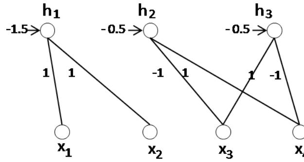
Figure 3.3: RBM for CIFFs.
