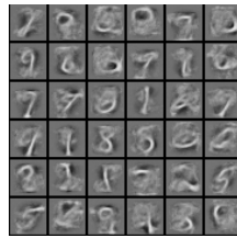
Figure 6.3: Representations (or feature detectors) from sparse RBMs learned on 20,000 MNIST samples.
