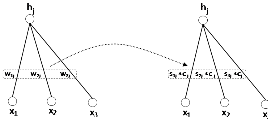
Figure 4.1: Converting a sub-network in original RBM to new sub-network in easy-to-interpret RBM.
