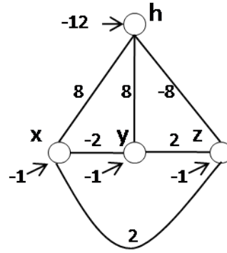
Figure 3.1: A Boltzmann machine for the XOR formula.
