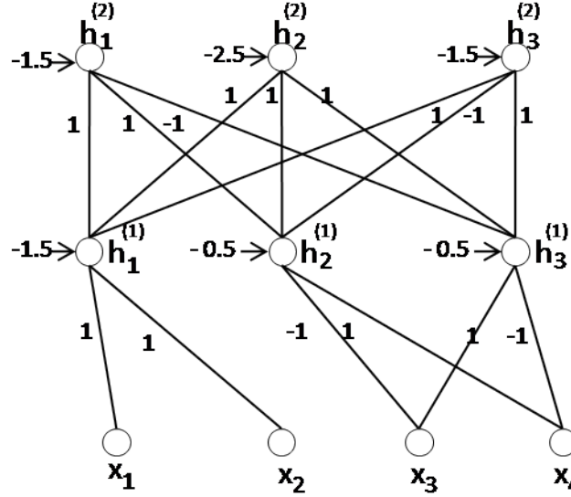
Figure 3.4: A DBN for x_1 \wedge x_2 \wedge (x_3 \oplus x_4) .
