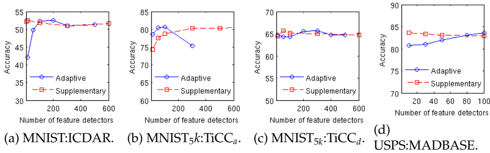
Figure 6.2: Number of complete-models/feature detectors in the adaptive part and in supplementary part of aTPL in four scenarios.
