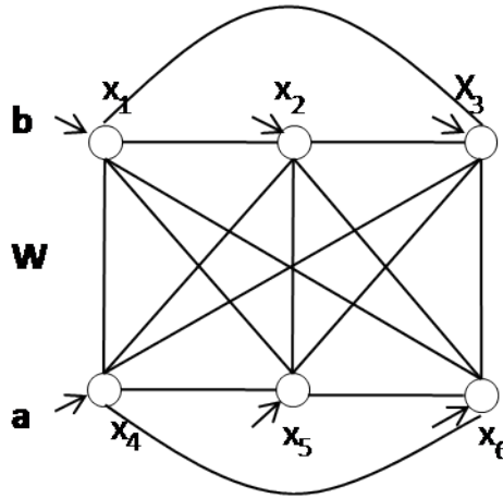
Figure 2.1: A Hopfield network ( \mathbf{s} = \{\mathbf{a}, \mathbf{b}\} ).
