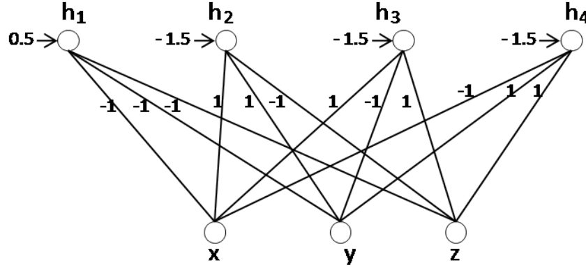
Figure 3.2: RBM for XOR formula: (x \oplus y) \leftrightarrow z .
