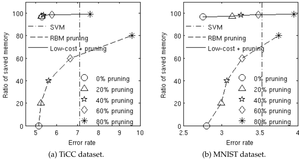
Figure 4.2: Error rate progression in comparison with memory capacity gains for RBMs and the extracted rules pruned by 0, 20, 40, 60 and 80%.
