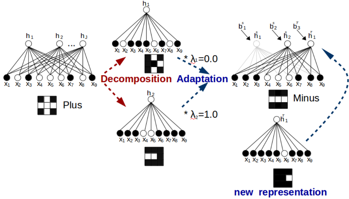
Figure 6.1: aTPL example of transferring representations from Plus image to Minus image.
