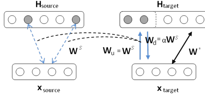
Figure 5.7: General representation transfer model for unsupervised learning.
