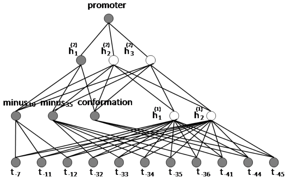
Figure 4.8: A deep neural-symbolic integration with 5 rules have been encoded.
