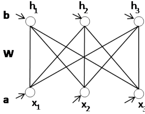
Figure 2.3: A restricted Boltzmann machine.
