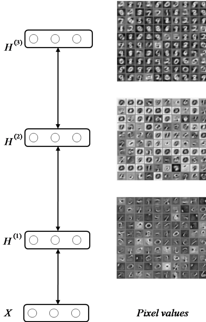
Figure 2.4: A stack of RBMs trained on handwritten digits with visualisations of the units in the hidden layers obtained by activating each hidden unit at a time and performing downward inference to the visible layer thus generating pixels for the images. The hierarchy is expected to model levels of abstraction by transforming the feature vectors, in this case from edges to shapes and finally digits.
