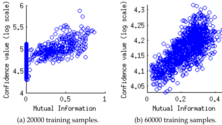
Figure 5.6: Mutual Information measurement on ranked feature detectors.
