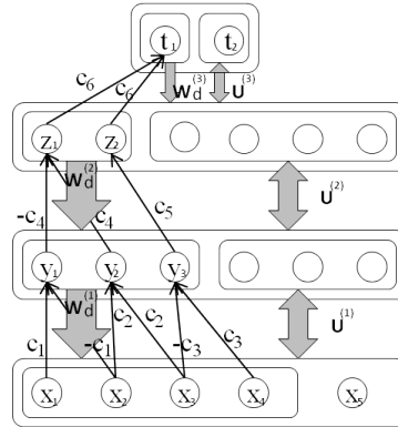
Figure 4.7: DBN obtained from hierarchical rule set K from Example 4.4.1.
