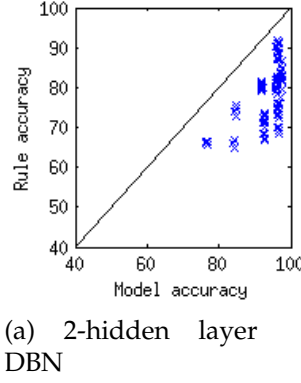
Figure 4.5: Comparison between the test-set accuracies of DBNs (model accuracy) and extracted rules.
