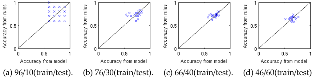
Figure 4.3: Classification performances of RBMs and the extracted rules on DNA promoter dataset.
