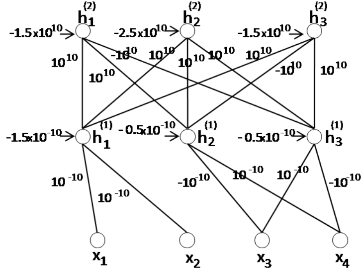
Figure 3.6: DBN corresponding to x_1 \wedge x_2 \wedge (x_3 \oplus x_4) .
