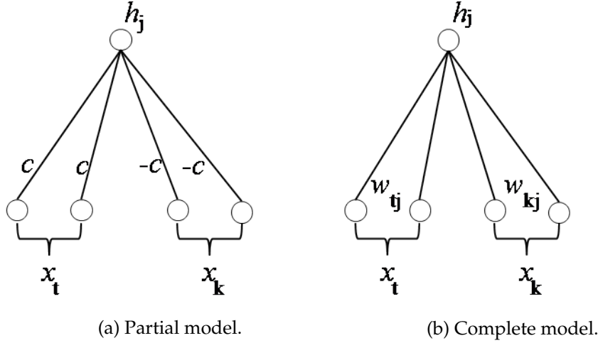
Figure 5.1: Sub-networks for partial model in Eq. 5.4 and complete model in Eq. 5.3, respectively. As we can see, the weights in the sub-network representing a partial model have the discrete values \{c, 0, -c\} , while the weights of the sub-network representing a complete model have real values, similar as the weights of RBMs.
