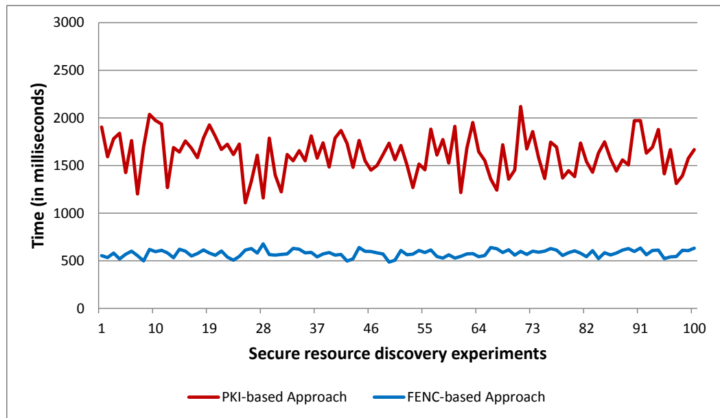
Figure 6.4: Secure resource discovery for 100 runtime trials between PKI and Functional Encryption based approaches in ICPN, between BT and ATOS cloud platform
