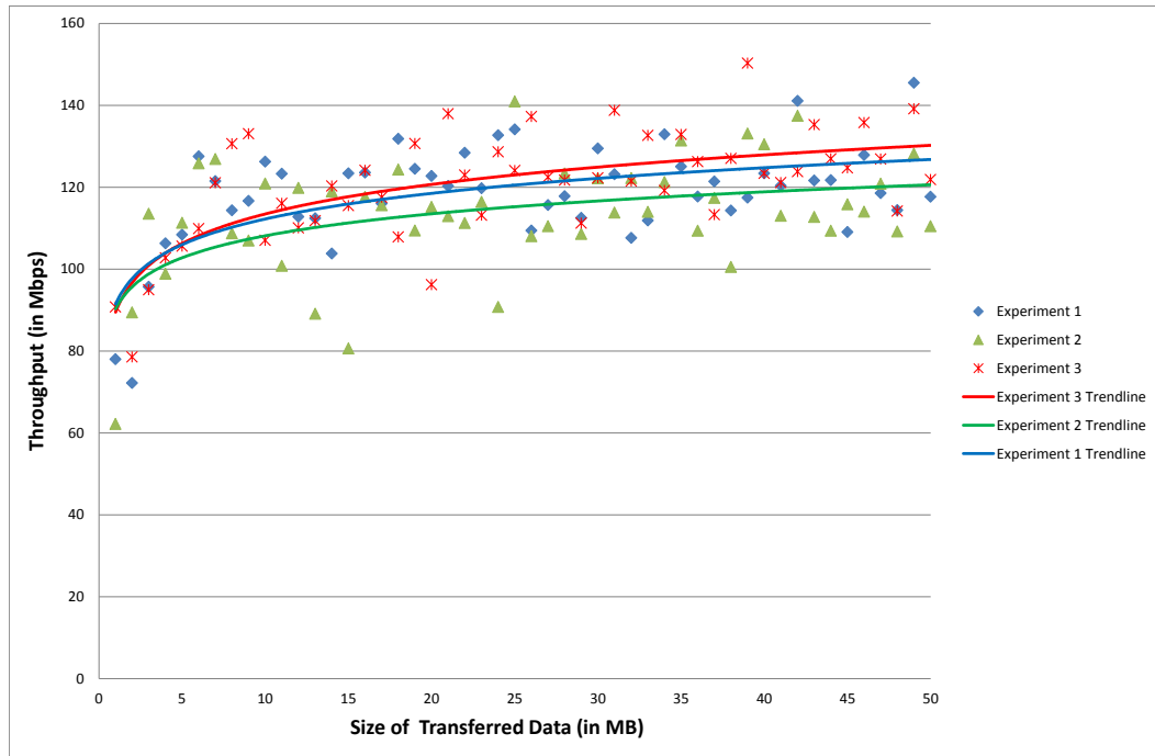
Figure 4.6: TPlot of 150 throughput measurements of 1-50 MB data transfers from Flexiant to BT clouds in order to find the most stable 3-tuple measurements
