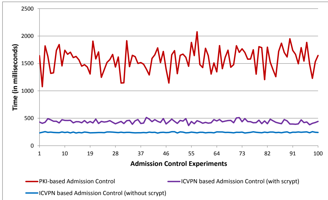
Figure 5.3: Duration of the admission control process for 100 trial instances using the PKI-based and ICPVPN methods, between BT and ATOS cloud platform
