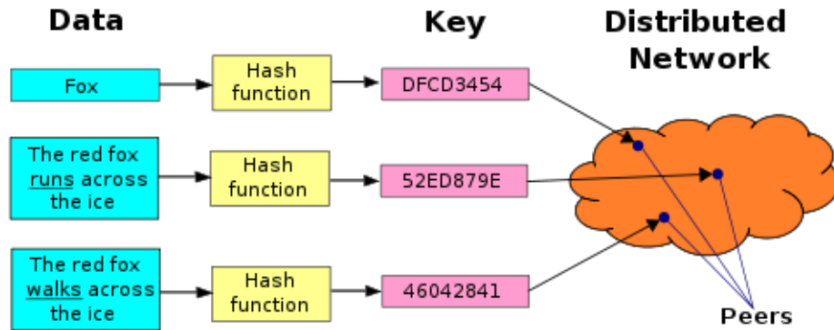
Figure 3.2: An operational description of a distributed hash table [162]
