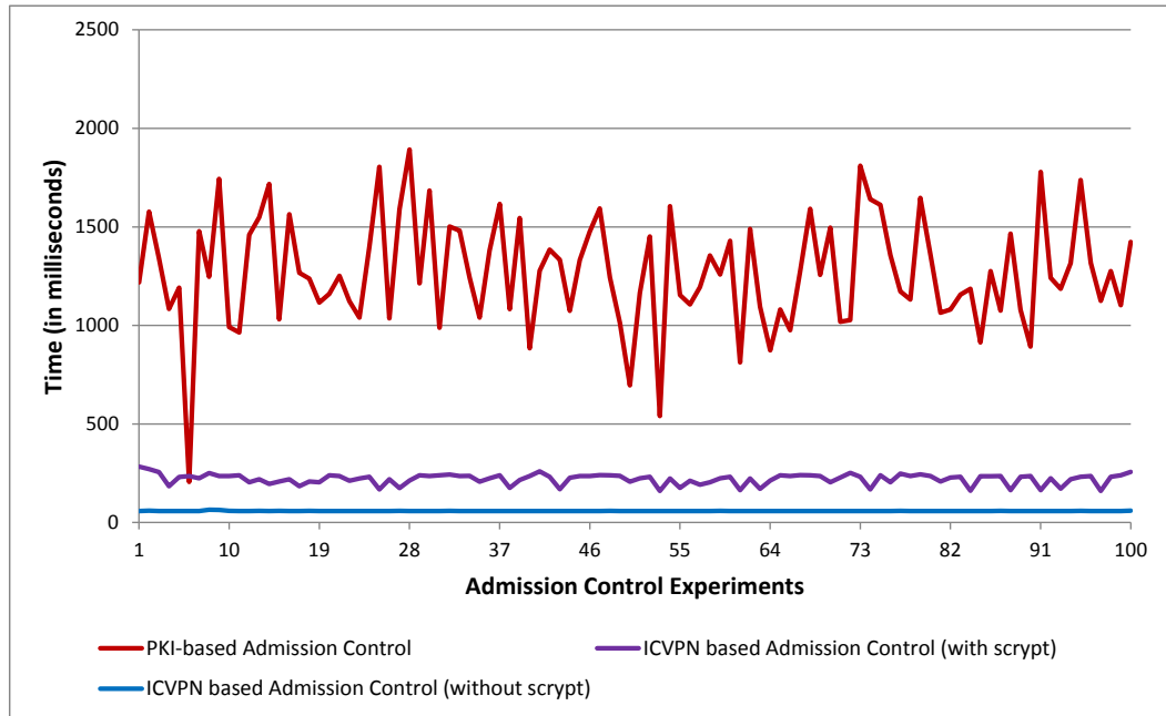
Figure 5.1: Duration of the admission control process for 100 trial instances using the PKI-based and ICPVPN methods, on a single cloud platform (BT)
