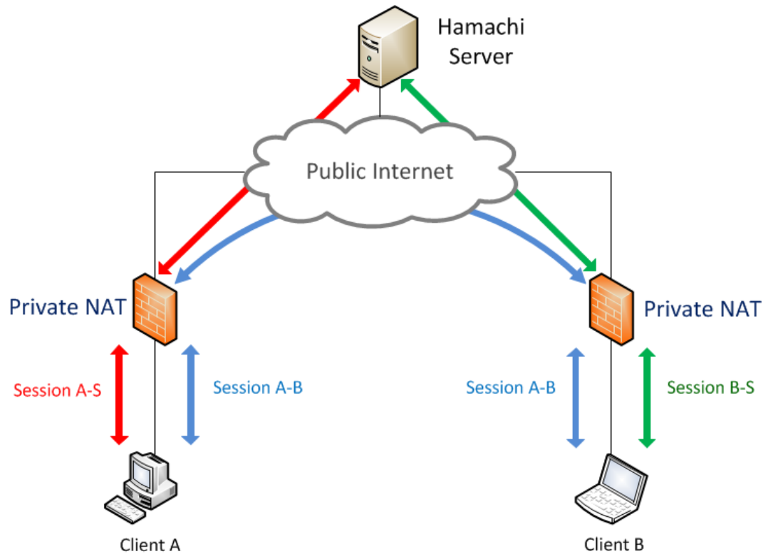
Figure 2.3: The Hamachi architecture for linking fire-walled peers. The fire-wall functionality is usually provided by private NAT devices that are transparent to the end-users of this service.
