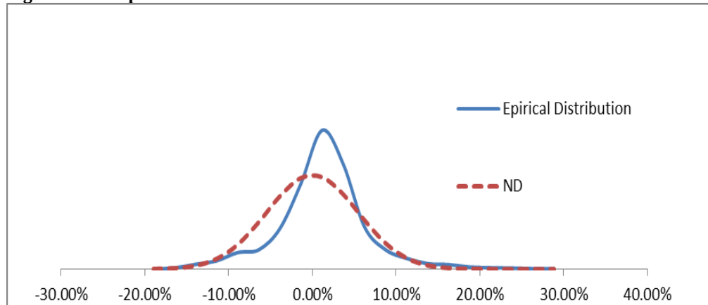
Figure 5-1: Empirical distribution
