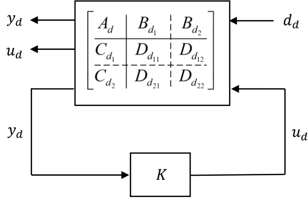
Figure 4.7.4 Discrete model
