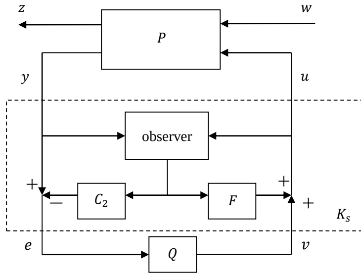
Figure 2.7.1 Interpretation of Q -parameterization for estimated state feedback K_s
